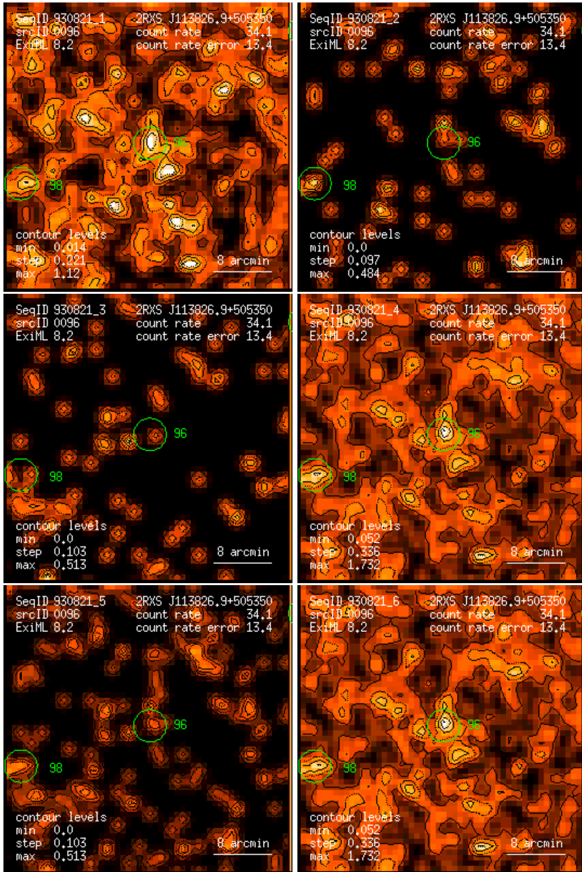
Figure 96: RASS 930821: detection 0096: band rate images, Gaussian filter: (1) PSPC channels 11 – 41, (2) 52 – 90, (3) 91 – 201, (4) 11 – 235, (5) 52 – 201, (6) 11 – 201. Broad band rates in counts/ks. Band rate contour levels in counts/ks/arcmin 2 .
