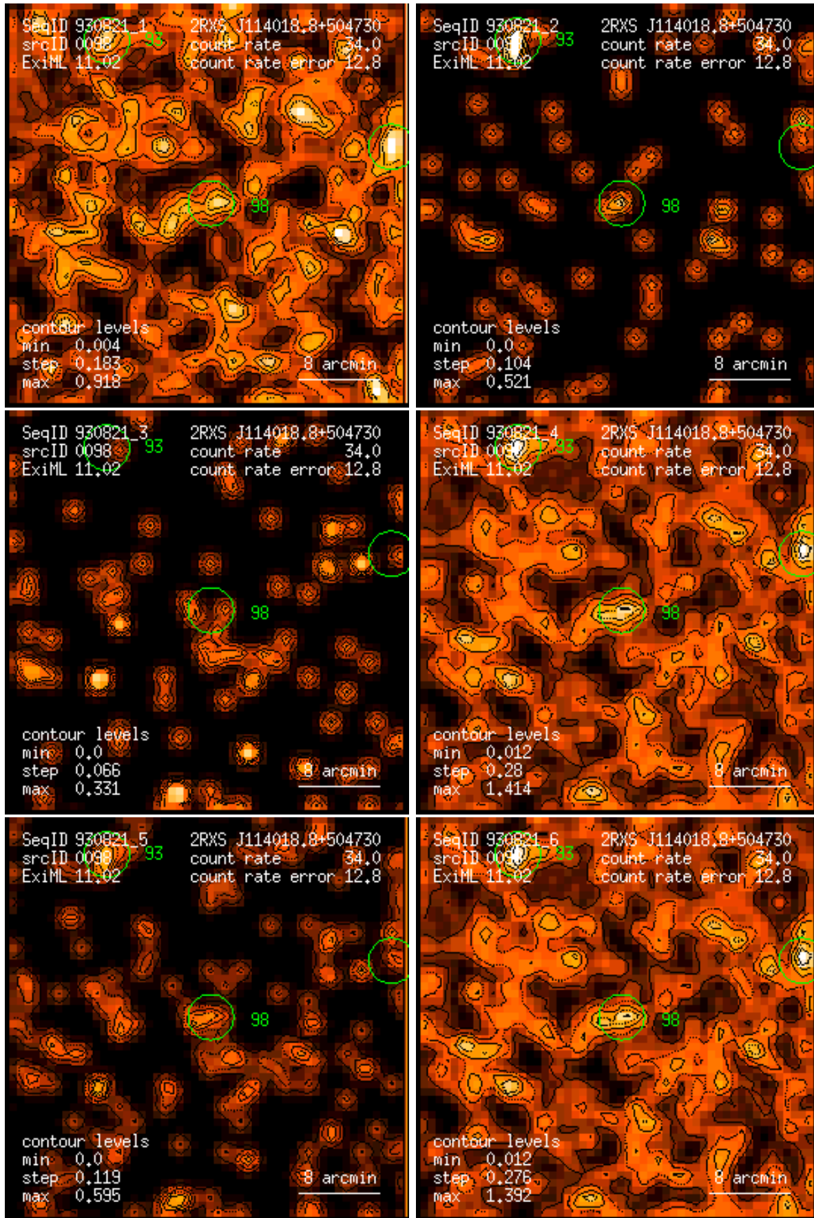
Figure 98: RASS 930821: detection 0098: band rate images, Gaussian filter: (1) PSPC channels 11 – 41, (2) 52 – 90, (3) 91 – 201, (4) 11 – 235, (5) 52 – 201, (6) 11 – 201. Broad band rates in counts/ks. Band rate contour levels in counts/ks/arcmin 2 .
