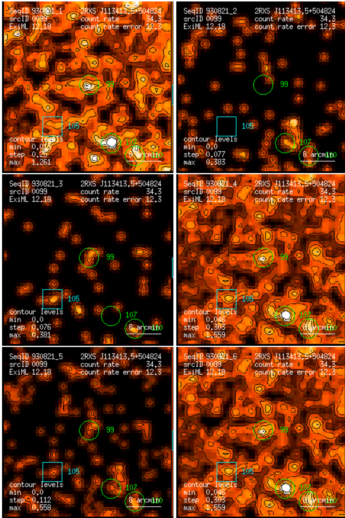
Figure 99: RASS 930821: detection 0099: band rate images, Gaussian filter: (1) PSPC channels 11 – 41, (2) 52 – 90, (3) 91 – 201, (4) 11 – 235, (5) 52 – 201, (6) 11 – 201. Broad band rates in counts/ks. Band rate contour levels in counts/ks/arcmin 2 .
