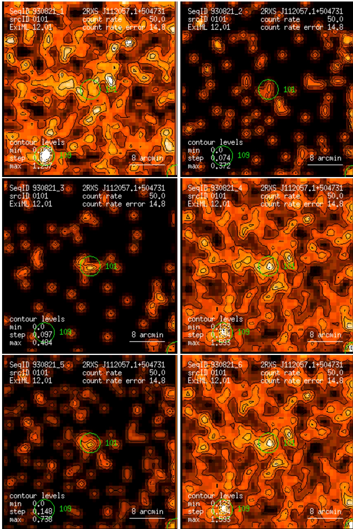
Figure 101: RASS 930821: detection 0101: band rate images, Gaussian filter: (1) PSPC channels 11 – 41, (2) 52 – 90, (3) 91 – 201, (4) 11 – 235, (5) 52 – 201, (6) 11 – 201. Broad band rates in counts/ks. Band rate contour levels in counts/ks/arcmin 2 .
