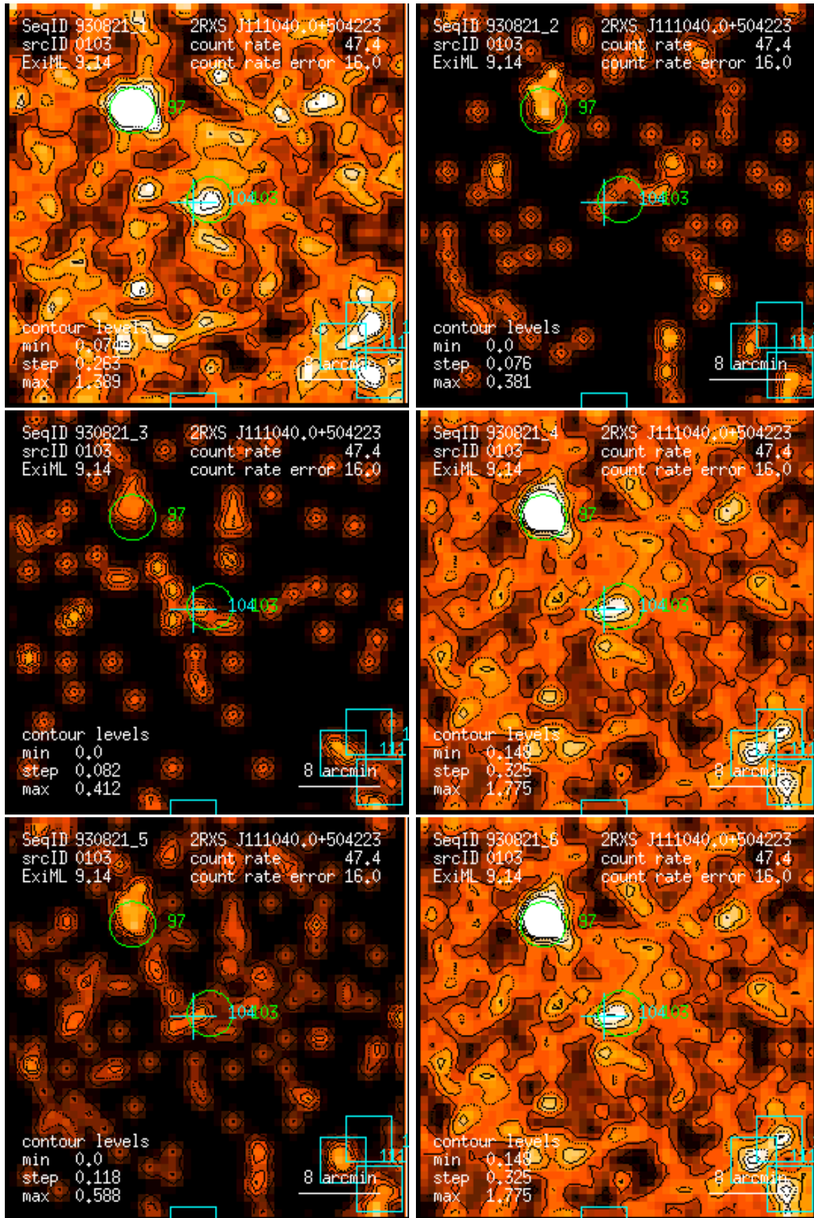
Figure 103: RASS 930821: detection 0103: band rate images, Gaussian filter: (1) PSPC channels 11 – 41, (2) 52 – 90, (3) 91 – 201, (4) 11 – 235, (5) 52 – 201, (6) 11 – 201. Broad band rates in counts/ks. Band rate contour levels in counts/ks/arcmin 2 .
