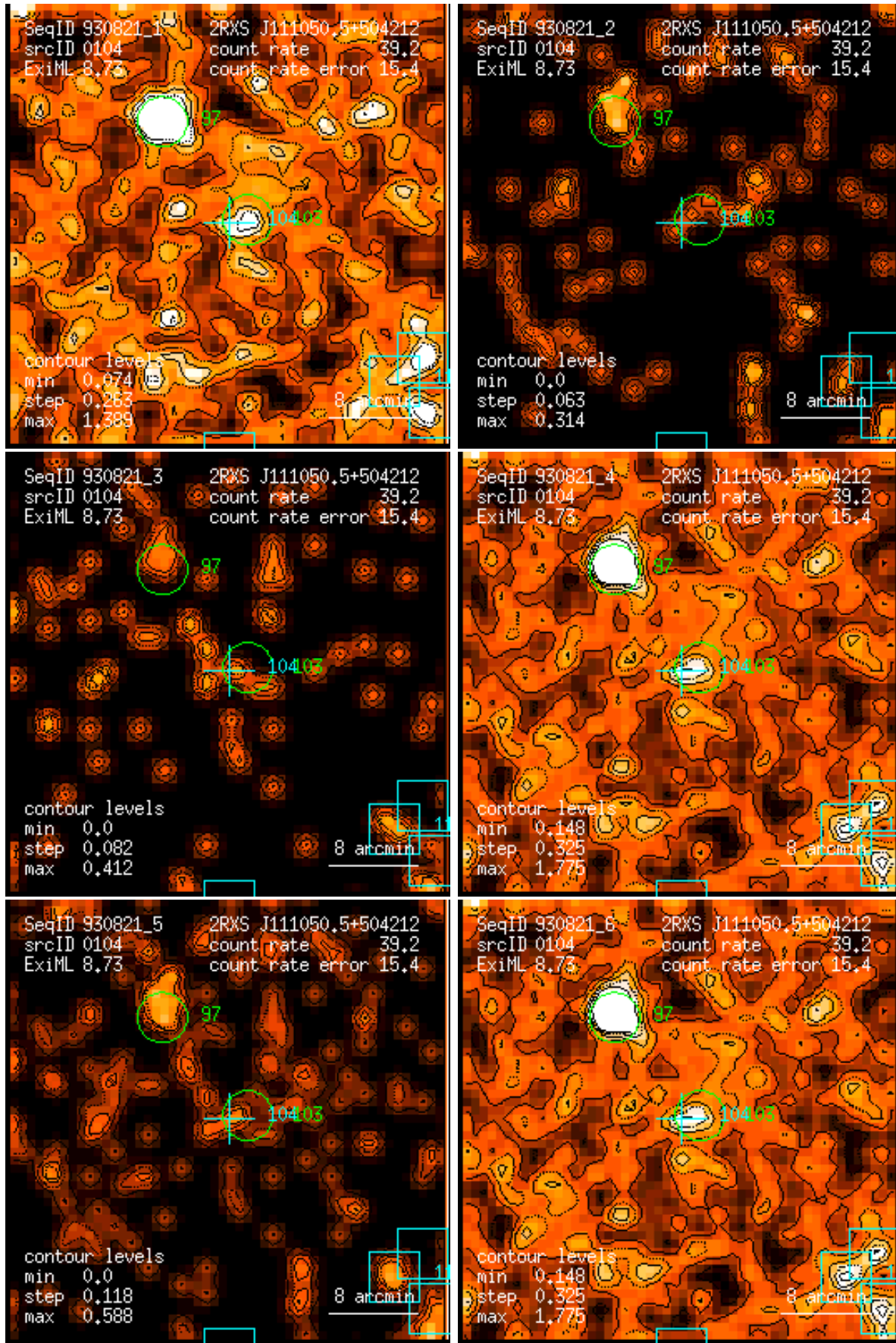
Figure 104: RASS 930821: detection 0104: band rate images, Gaussian filter: (1) PSPC channels 11 – 41, (2) 52 – 90, (3) 91 – 201, (4) 11 – 235, (5) 52 – 201, (6) 11 – 201. Broad band rates in counts/ks. Band rate contour levels in counts/ks/arcmin 2 .
