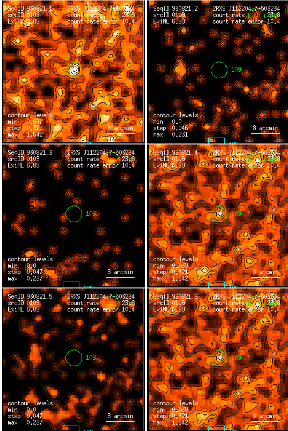
Figure 109: RASS 930821: detection 0109: band rate images, Gaussian filter: (1) PSPC channels 11 – 41, (2) 52 – 90, (3) 91 – 201, (4) 11 – 235, (5) 52 – 201, (6) 11 – 201. Broad band rates in counts/ks. Band rate contour levels in counts/ks/arcmin 2 .
