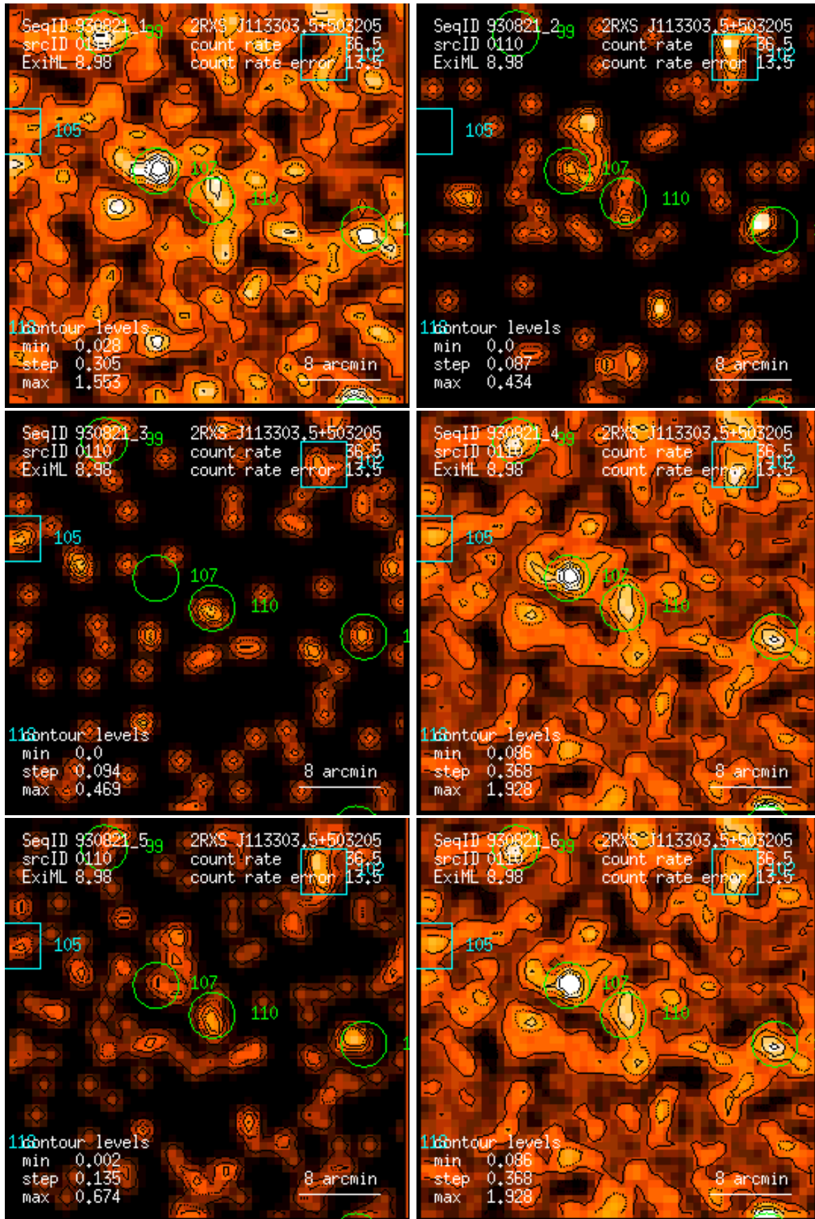
Figure 110: RASS 930821: detection 0110: band rate images, Gaussian filter: (1) PSPC channels 11 – 41, (2) 52 – 90, (3) 91 – 201, (4) 11 – 235, (5) 52 – 201, (6) 11 – 201. Broad band rates in counts/ks. Band rate contour levels in counts/ks/arcmin 2 .
