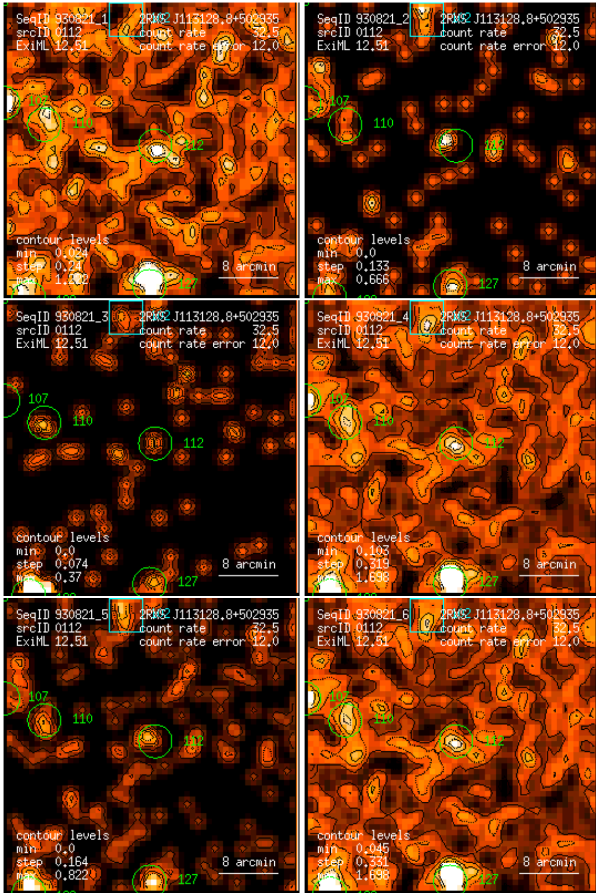
Figure 112: RASS 930821: detection 0112: band rate images, Gaussian filter: (1) PSPC channels 11 – 41, (2) 52 – 90, (3) 91 – 201, (4) 11 – 235, (5) 52 – 201, (6) 11 – 201. Broad band rates in counts/ks. Band rate contour levels in counts/ks/arcmin 2 .
