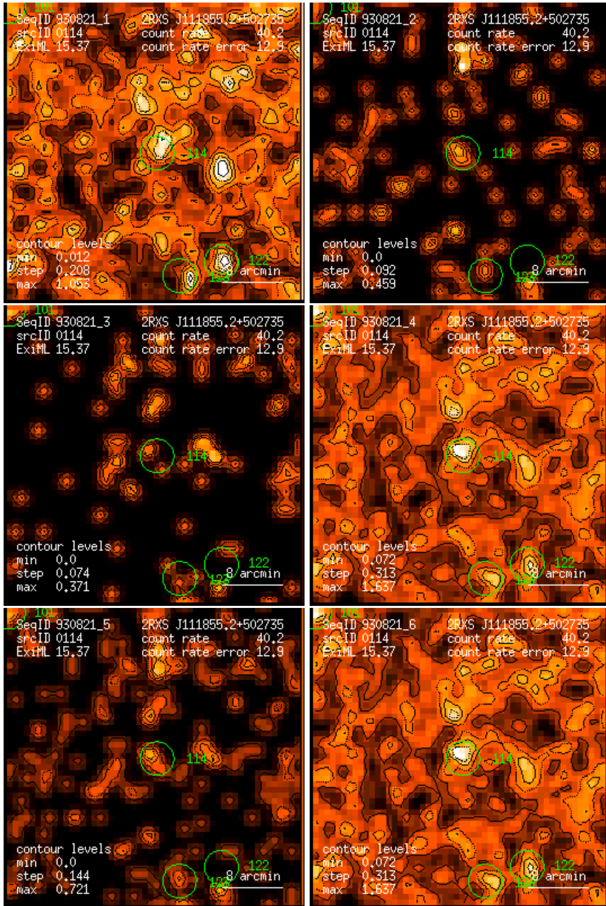
Figure 114: RASS 930821: detection 0114: band rate images, Gaussian filter: (1) PSPC channels 11 – 41, (2) 52 – 90, (3) 91 – 201, (4) 11 – 235, (5) 52 – 201, (6) 11 – 201. Broad band rates in counts/ks. Band rate contour levels in counts/ks/arcmin 2 .
