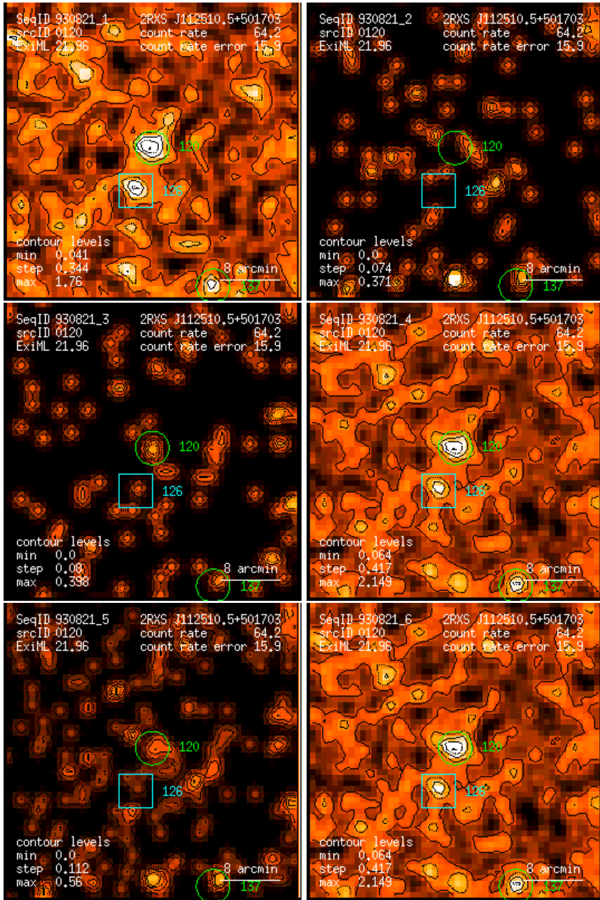
Figure 120: RASS 930821: detection 0120: band rate images, Gaussian filter: (1) PSPC channels 11 – 41, (2) 52 – 90, (3) 91 – 201, (4) 11 – 235, (5) 52 – 201, (6) 11 – 201. Broad band rates in counts/ks. Band rate contour levels in counts/ks/arcmin 2 .
