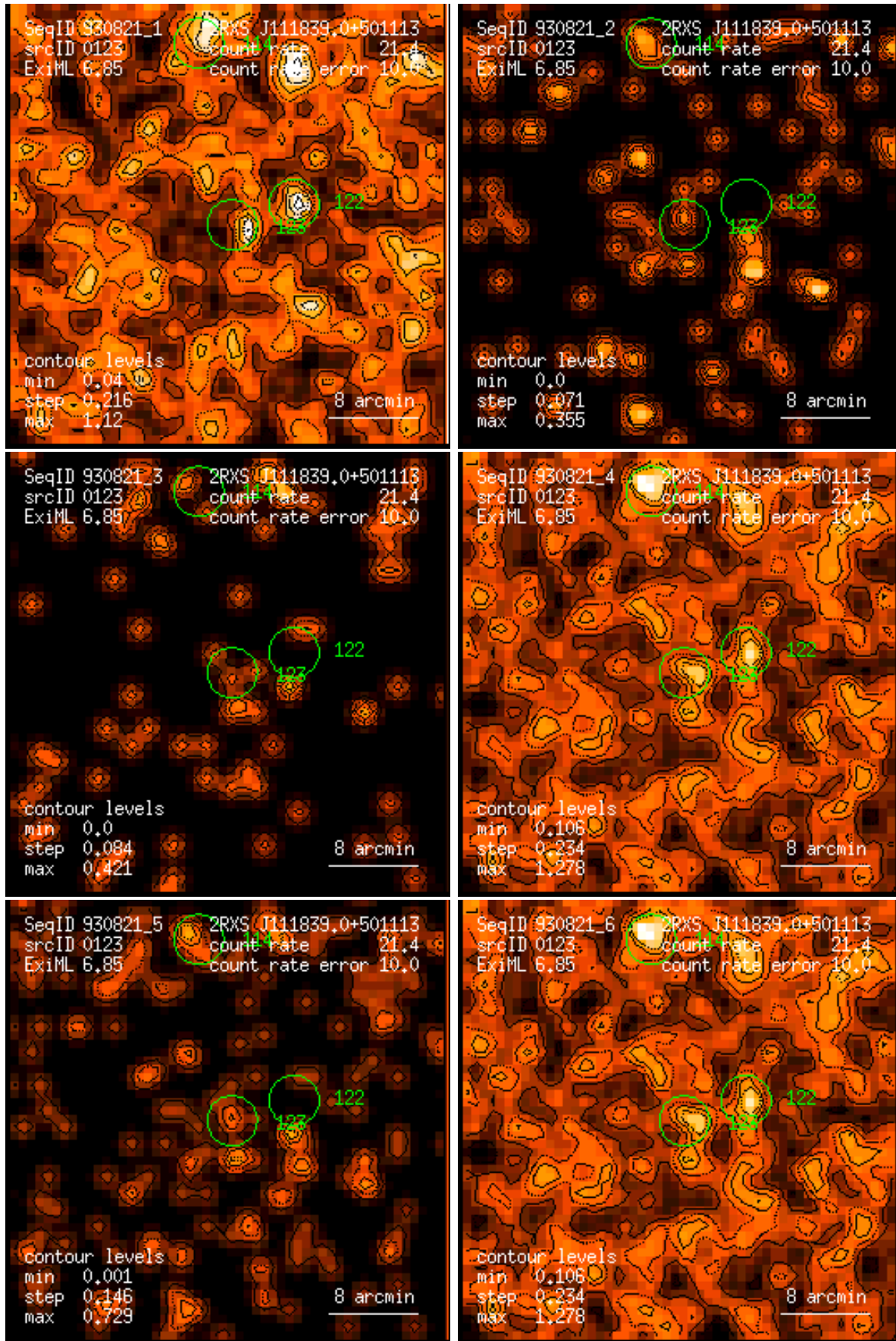
Figure 123: RASS 930821: detection 0123: band rate images, Gaussian filter: (1) PSPC channels 11 – 41, (2) 52 – 90, (3) 91 – 201, (4) 11 – 235, (5) 52 – 201, (6) 11 – 201. Broad band rates in counts/ks. Band rate contour levels in counts/ks/arcmin 2 .
