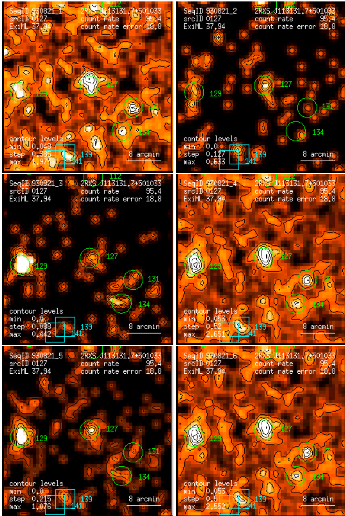
Figure 127: RASS 930821: detection 0127: band rate images, Gaussian filter: (1) PSPC channels 11 – 41, (2) 52 – 90, (3) 91 – 201, (4) 11 – 235, (5) 52 – 201, (6) 11 – 201. Broad band rates in counts/ks. Band rate contour levels in counts/ks/arcmin 2 .
