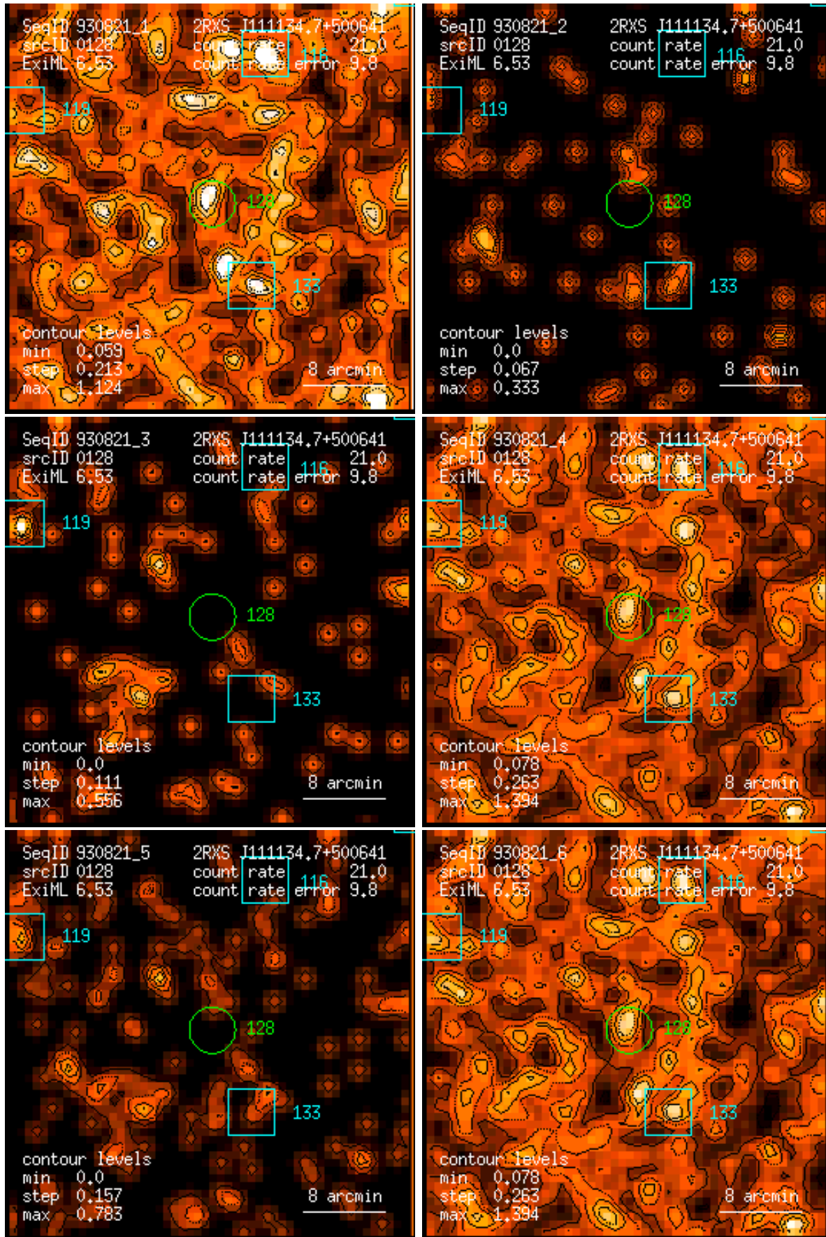
Figure 128: RASS 930821: detection 0128: band rate images, Gaussian filter: (1) PSPC channels 11 – 41, (2) 52 – 90, (3) 91 – 201, (4) 11 – 235, (5) 52 – 201, (6) 11 – 201. Broad band rates in counts/ks. Band rate contour levels in counts/ks/arcmin 2 .
