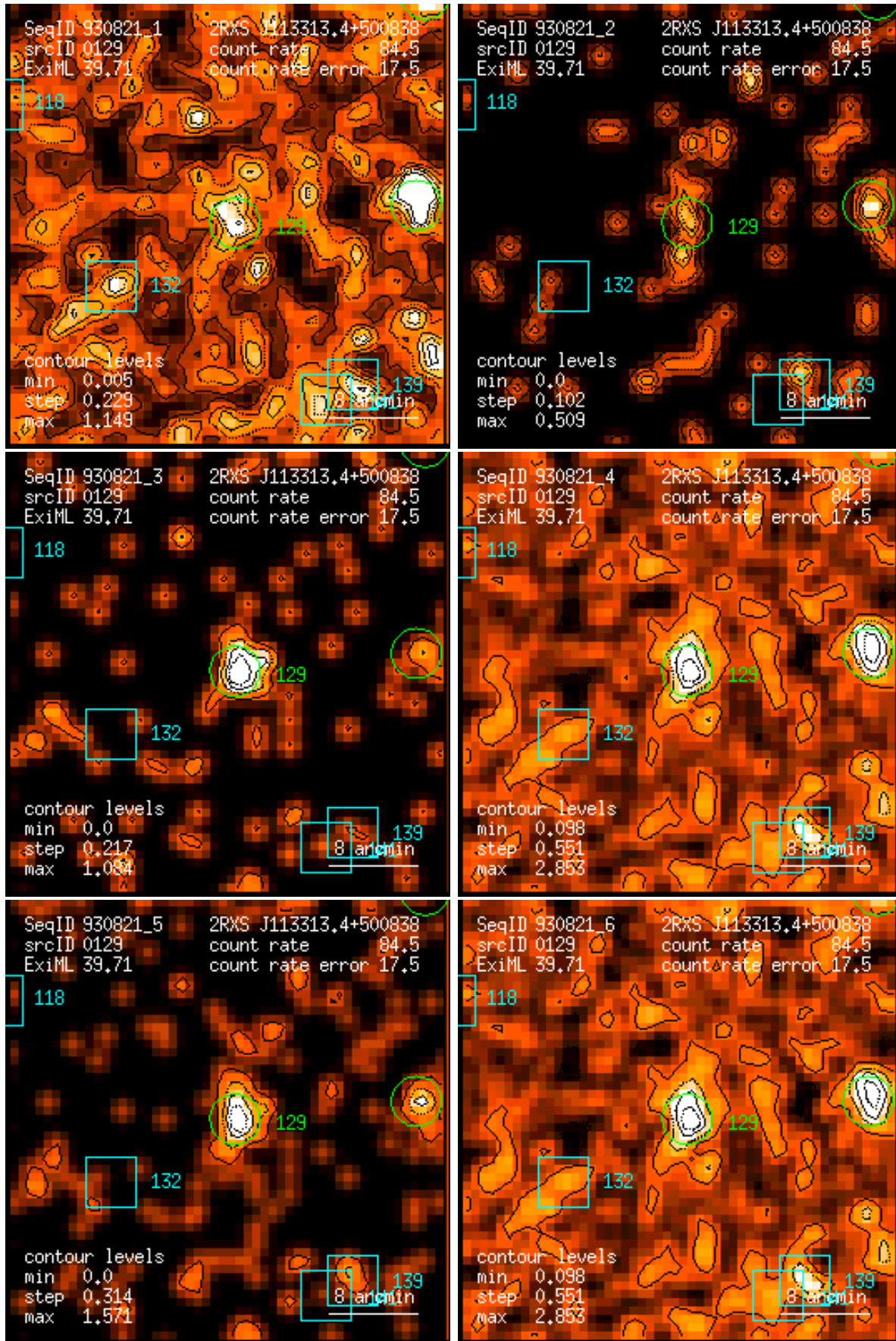
Figure 129: RASS 930821: detection 0129: band rate images, Gaussian filter: (1) PSPC channels 11 – 41, (2) 52 – 90, (3) 91 – 201, (4) 11 – 235, (5) 52 – 201, (6) 11 – 201. Broad band rates in counts/ks. Band rate contour levels in counts/ks/arcmin 2 .
