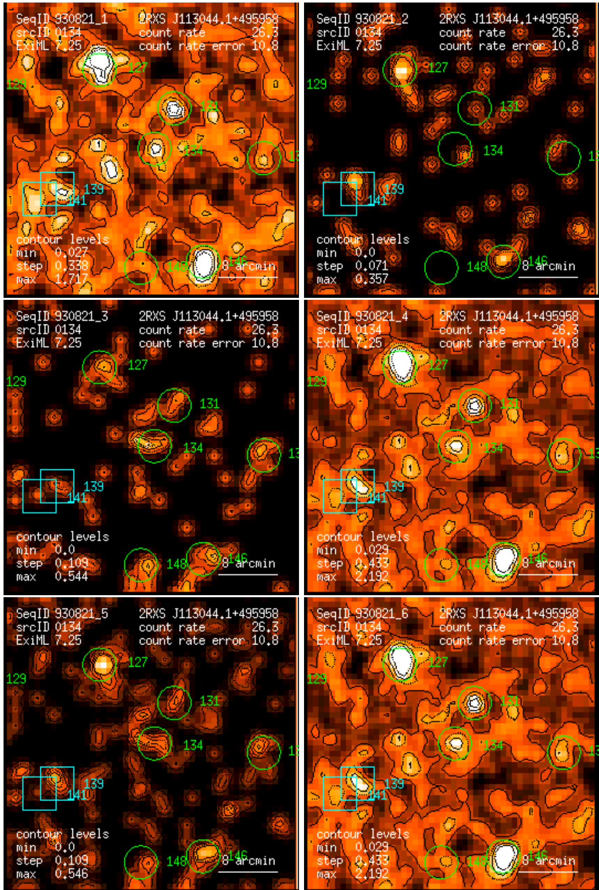
Figure 134: RASS 930821: detection 0134: band rate images, Gaussian filter: (1) PSPC channels 11 – 41, (2) 52 – 90, (3) 91 – 201, (4) 11 – 235, (5) 52 – 201, (6) 11 – 201. Broad band rates in counts/ks. Band rate contour levels in counts/ks/arcmin 2 .
