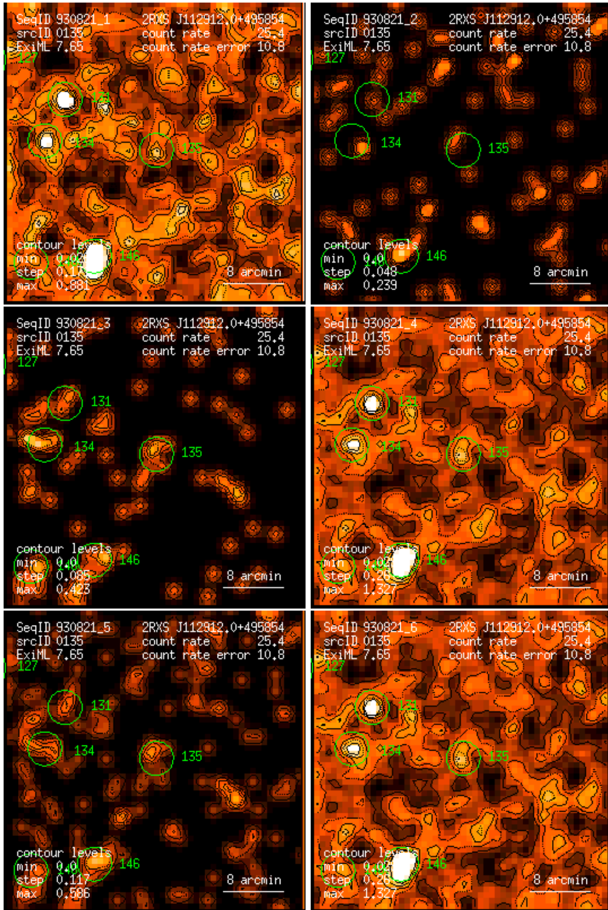
Figure 135: RASS 930821: detection 0135: band rate images, Gaussian filter: (1) PSPC channels 11 – 41, (2) 52 – 90, (3) 91 – 201, (4) 11 – 235, (5) 52 – 201, (6) 11 – 201. Broad band rates in counts/ks. Band rate contour levels in counts/ks/arcmin 2 .
