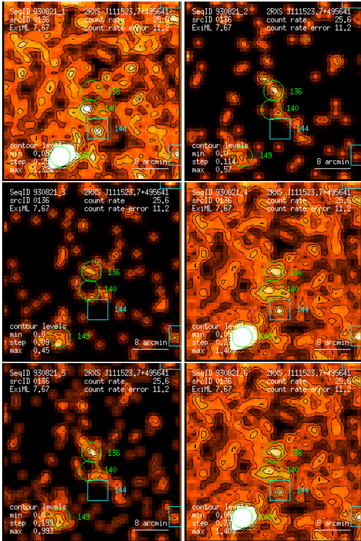
Figure 136: RASS 930821: detection 0136: band rate images, Gaussian filter: (1) PSPC channels 11 – 41, (2) 52 – 90, (3) 91 – 201, (4) 11 – 235, (5) 52 – 201, (6) 11 – 201. Broad band rates in counts/ks. Band rate contour levels in counts/ks/arcmin 2 .
