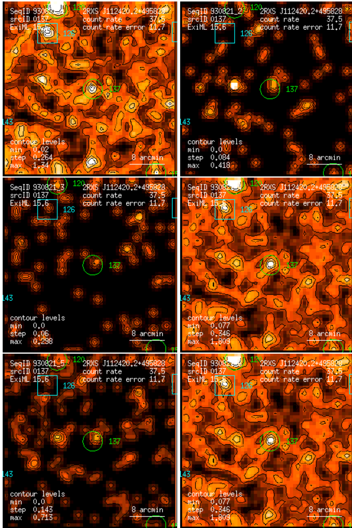
Figure 137: RASS 930821: detection 0137: band rate images, Gaussian filter: (1) PSPC channels 11 – 41, (2) 52 – 90, (3) 91 – 201, (4) 11 – 235, (5) 52 – 201, (6) 11 – 201. Broad band rates in counts/ks. Band rate contour levels in counts/ks/arcmin 2 .
