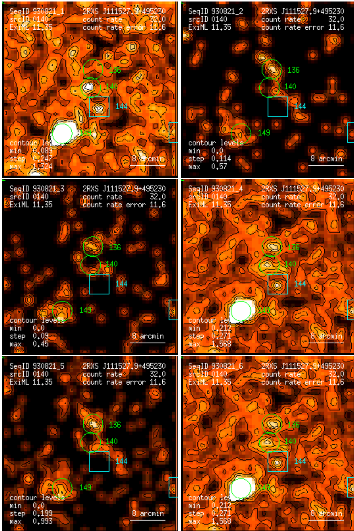
Figure 140: RASS 930821: detection 0140: band rate images, Gaussian filter: (1) PSPC channels 11 – 41, (2) 52 – 90, (3) 91 – 201, (4) 11 – 235, (5) 52 – 201, (6) 11 – 201. Broad band rates in counts/ks. Band rate contour levels in counts/ks/arcmin 2 .
