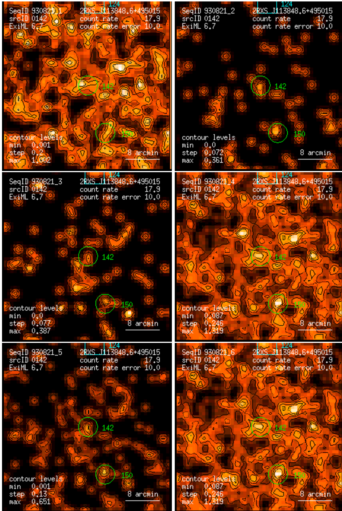
Figure 142: RASS 930821: detection 0142: band rate images, Gaussian filter: (1) PSPC channels 11 – 41, (2) 52 – 90, (3) 91 – 201, (4) 11 – 235, (5) 52 – 201, (6) 11 – 201. Broad band rates in counts/ks. Band rate contour levels in counts/ks/arcmin 2 .
