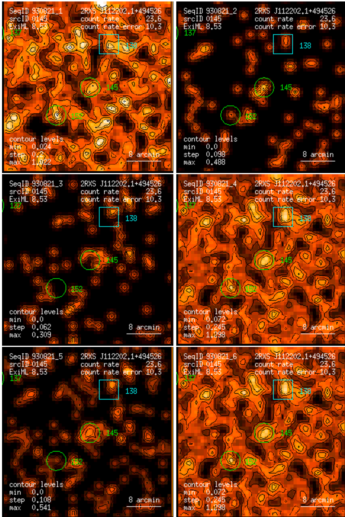
Figure 145: RASS 930821: detection 0145: band rate images, Gaussian filter: (1) PSPC channels 11 – 41, (2) 52 – 90, (3) 91 – 201, (4) 11 – 235, (5) 52 – 201, (6) 11 – 201. Broad band rates in counts/ks. Band rate contour levels in counts/ks/arcmin 2 .
