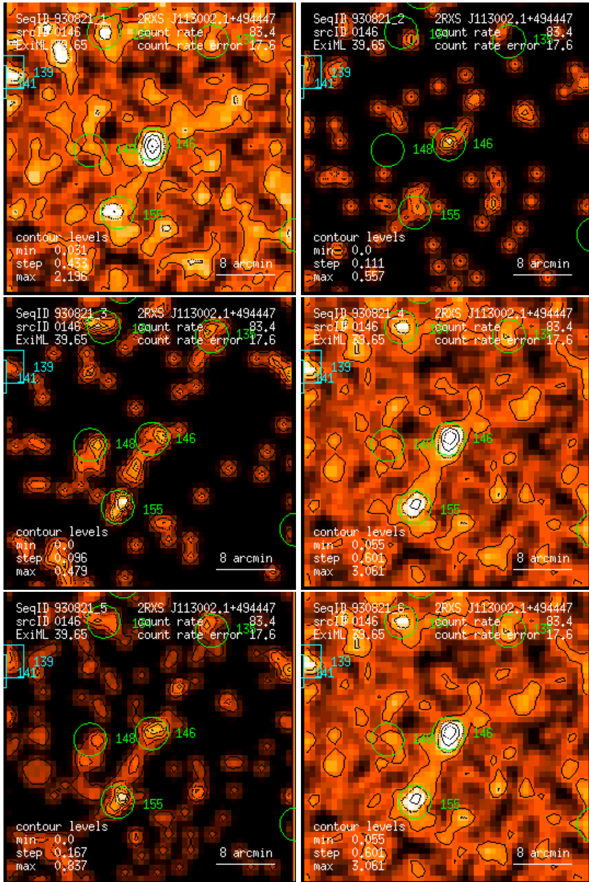
Figure 146: RASS 930821: detection 0146: band rate images, Gaussian filter: (1) PSPC channels 11 – 41, (2) 52 – 90, (3) 91 – 201, (4) 11 – 235, (5) 52 – 201, (6) 11 – 201. Broad band rates in counts/ks. Band rate contour levels in counts/ks/arcmin 2 .
