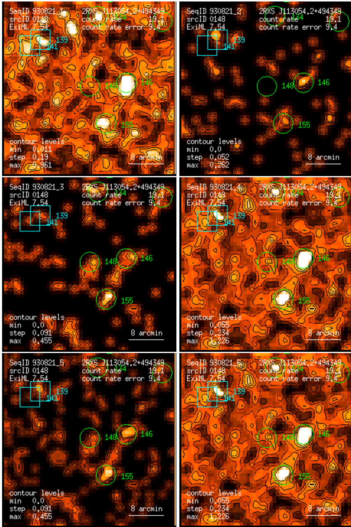
Figure 148: RASS 930821: detection 0148: band rate images, Gaussian filter: (1) PSPC channels 11 – 41, (2) 52 – 90, (3) 91 – 201, (4) 11 – 235, (5) 52 – 201, (6) 11 – 201. Broad band rates in counts/ks. Band rate contour levels in counts/ks/arcmin 2 .
