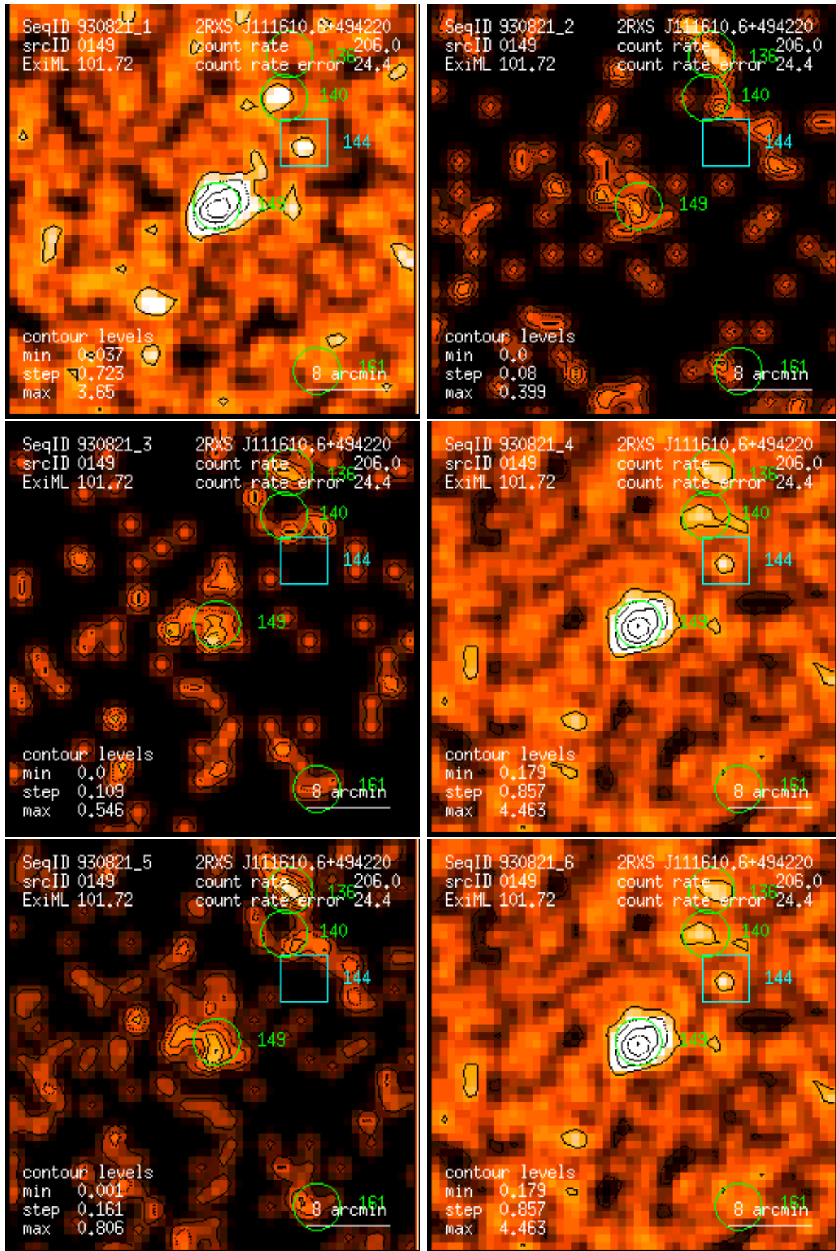
Figure 149: RASS 930821: detection 0149: band rate images, Gaussian filter: (1) PSPC channels 11 – 41, (2) 52 – 90, (3) 91 – 201, (4) 11 – 235, (5) 52 – 201, (6) 11 – 201. Broad band rates in counts/ks. Band rate contour levels in counts/ks/arcmin 2 .
