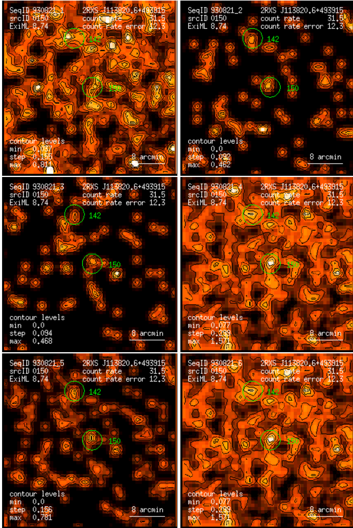
Figure 150: RASS 930821: detection 0150: band rate images, Gaussian filter: (1) PSPC channels 11 – 41, (2) 52 – 90, (3) 91 – 201, (4) 11 – 235, (5) 52 – 201, (6) 11 – 201. Broad band rates in counts/ks. Band rate contour levels in counts/ks/arcmin 2 .
