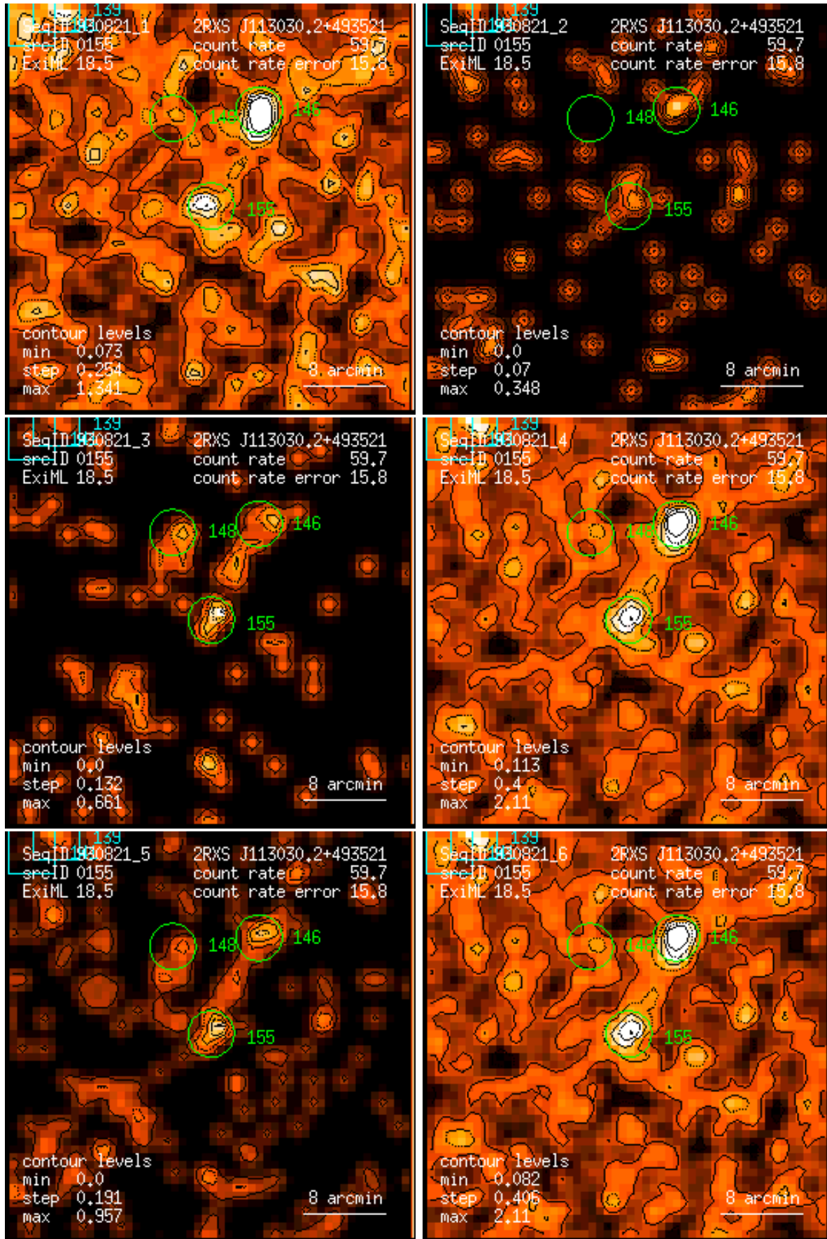
Figure 155: RASS 930821: detection 0155: band rate images, Gaussian filter: (1) PSPC channels 11 – 41, (2) 52 – 90, (3) 91 – 201, (4) 11 – 235, (5) 52 – 201, (6) 11 – 201. Broad band rates in counts/ks. Band rate contour levels in counts/ks/arcmin 2 .
