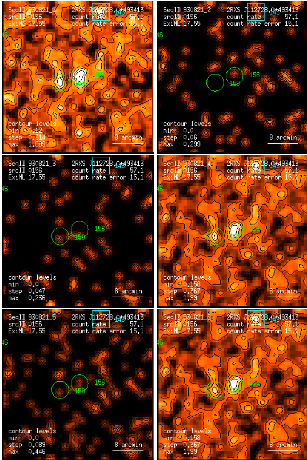
Figure 156: RASS 930821: detection 0156: band rate images, Gaussian filter: (1) PSPC channels 11 – 41, (2) 52 – 90, (3) 91 – 201, (4) 11 – 235, (5) 52 – 201, (6) 11 – 201. Broad band rates in counts/ks. Band rate contour levels in counts/ks/arcmin 2 .
