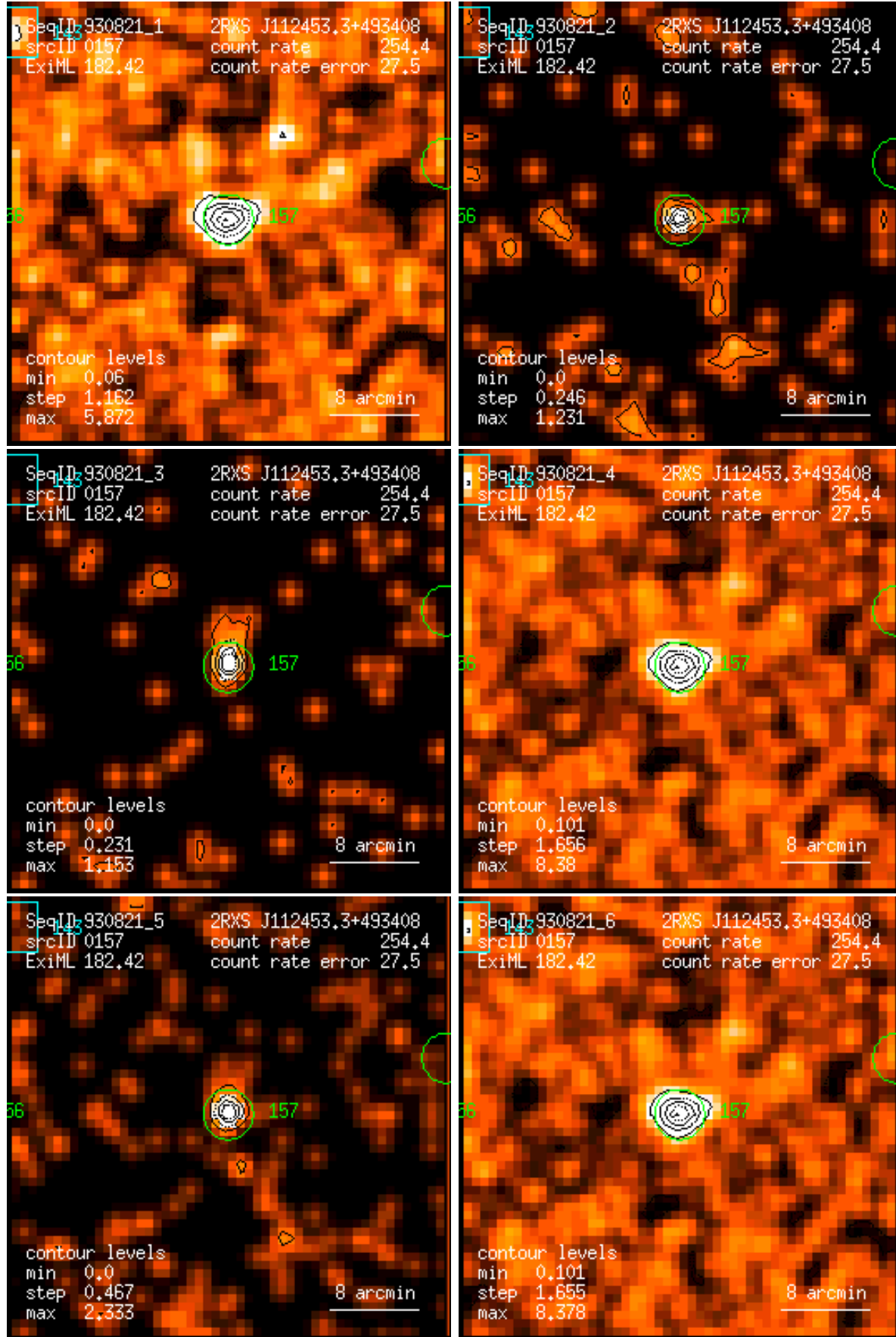
Figure 157: RASS 930821: detection 0157: band rate images, Gaussian filter: (1) PSPC channels 11 – 41, (2) 52 – 90, (3) 91 – 201, (4) 11 – 235, (5) 52 – 201, (6) 11 – 201. Broad band rates in counts/ks. Band rate contour levels in counts/ks/arcmin 2 .
