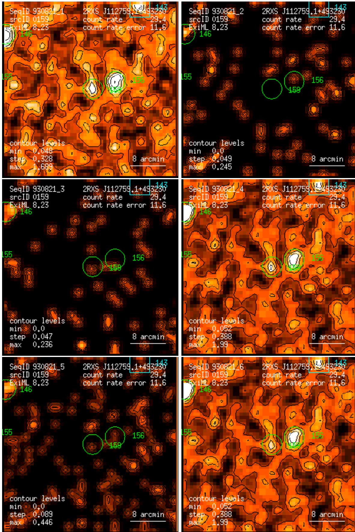
Figure 159: RASS 930821: detection 0159: band rate images, Gaussian filter: (1) PSPC channels 11 – 41, (2) 52 – 90, (3) 91 – 201, (4) 11 – 235, (5) 52 – 201, (6) 11 – 201. Broad band rates in counts/ks. Band rate contour levels in counts/ks/arcmin 2 .
