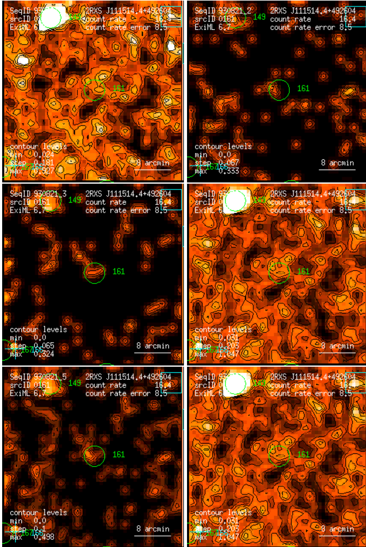
Figure 161: RASS 930821: detection 0161: band rate images, Gaussian filter: (1) PSPC channels 11 – 41, (2) 52 – 90, (3) 91 – 201, (4) 11 – 235, (5) 52 – 201, (6) 11 – 201. Broad band rates in counts/ks. Band rate contour levels in counts/ks/arcmin 2 .
