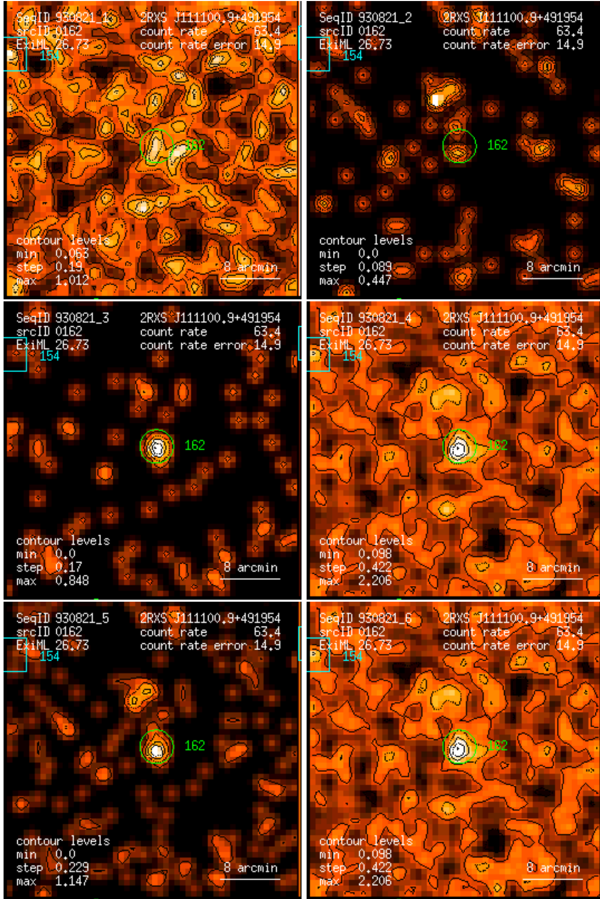
Figure 162: RASS 930821: detection 0162: band rate images, Gaussian filter: (1) PSPC channels 11 – 41, (2) 52 – 90, (3) 91 – 201, (4) 11 – 235, (5) 52 – 201, (6) 11 – 201. Broad band rates in counts/ks. Band rate contour levels in counts/ks/arcmin 2 .
