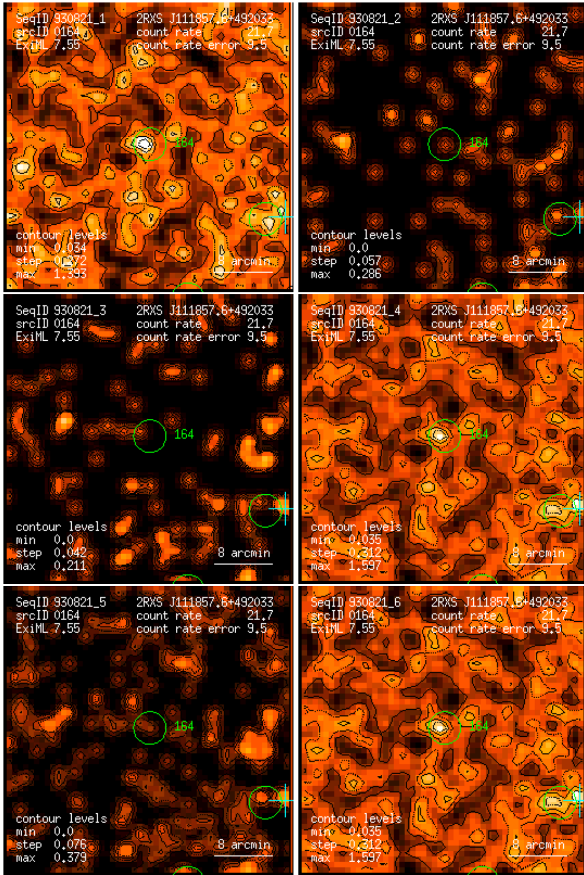
Figure 164: RASS 930821: detection 0164: band rate images, Gaussian filter: (1) PSPC channels 11 – 41, (2) 52 – 90, (3) 91 – 201, (4) 11 – 235, (5) 52 – 201, (6) 11 – 201. Broad band rates in counts/ks. Band rate contour levels in counts/ks/arcmin 2 .
