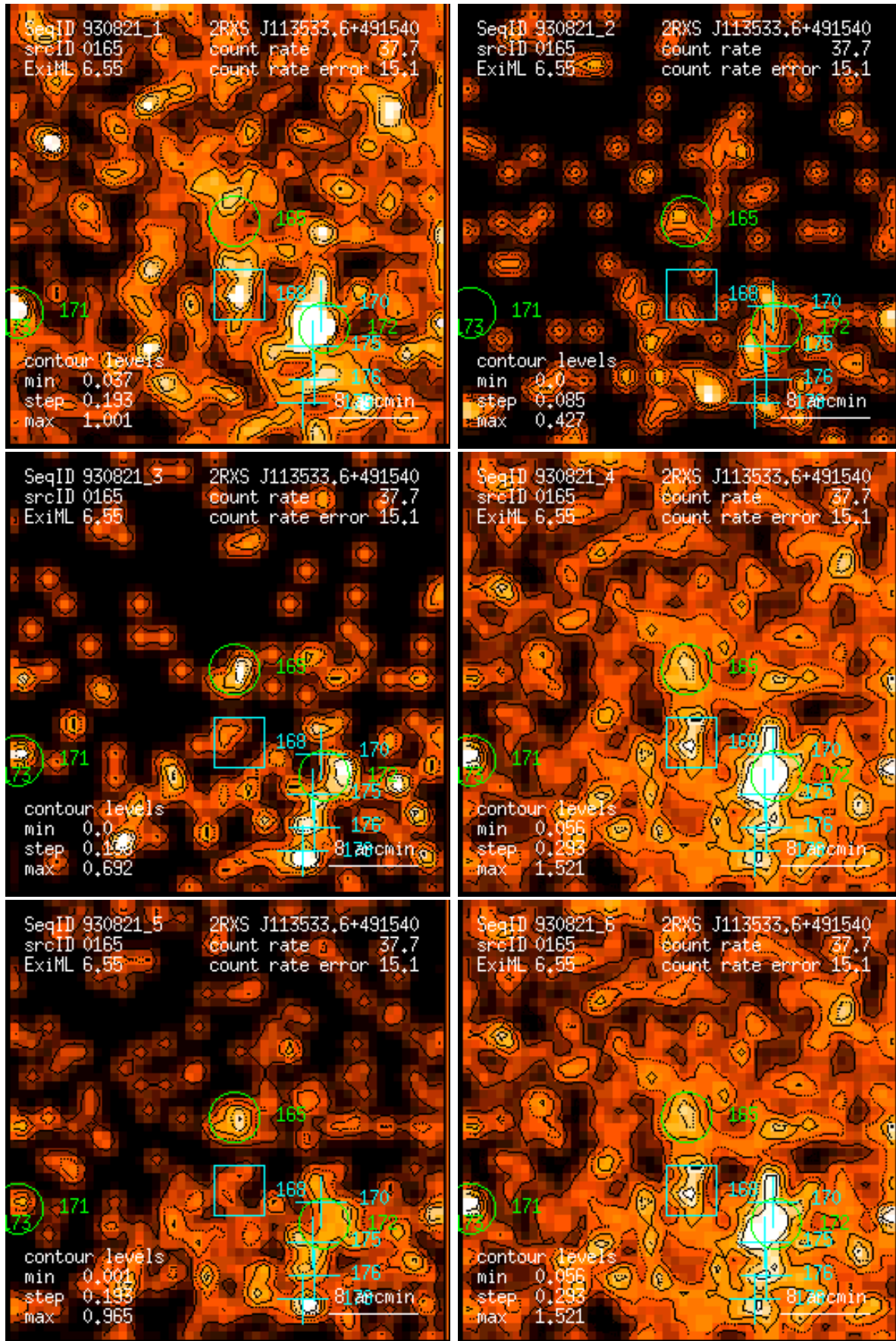
Figure 165: RASS 930821: detection 0165: band rate images, Gaussian filter: (1) PSPC channels 11 – 41, (2) 52 – 90, (3) 91 – 201, (4) 11 – 235, (5) 52 – 201, (6) 11 – 201. Broad band rates in counts/ks. Band rate contour levels in counts/ks/arcmin 2 .
