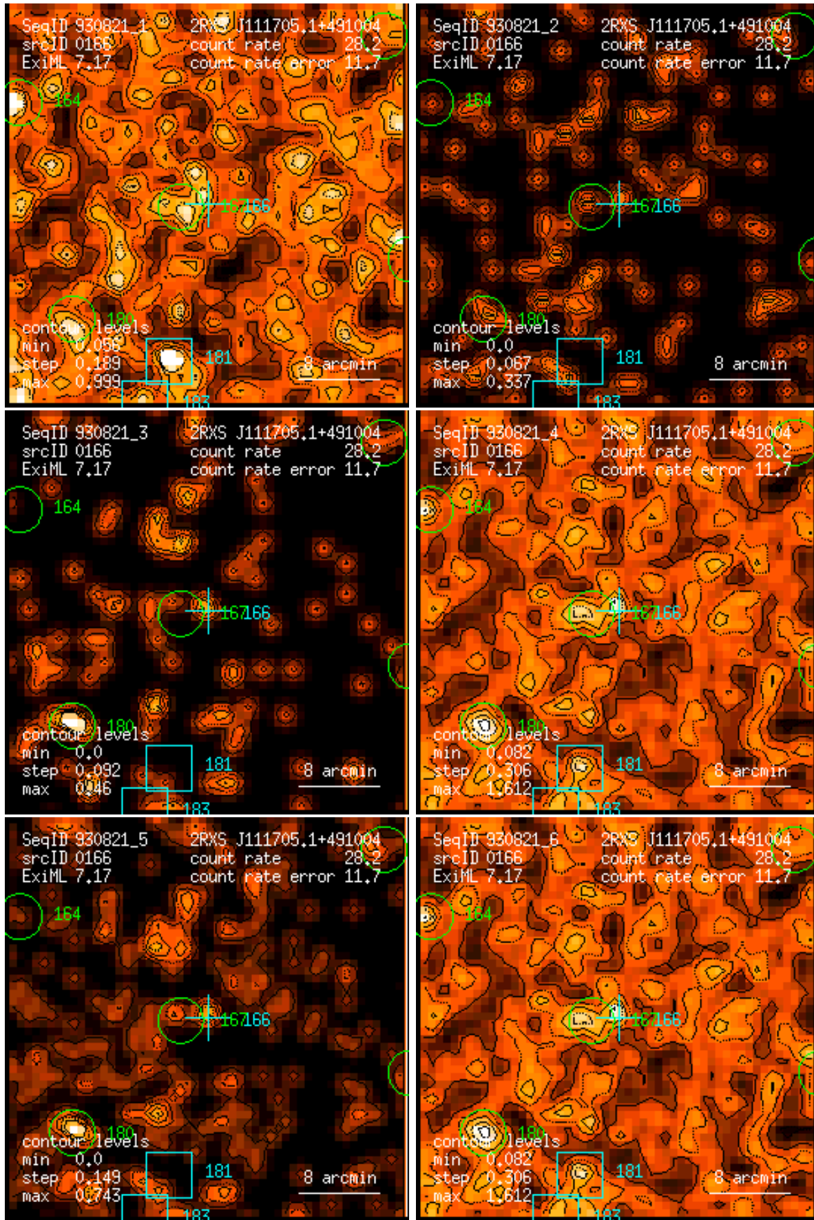
Figure 166: RASS 930821: detection 0166: band rate images, Gaussian filter: (1) PSPC channels 11 – 41, (2) 52 – 90, (3) 91 – 201, (4) 11 – 235, (5) 52 – 201, (6) 11 – 201. Broad band rates in counts/ks. Band rate contour levels in counts/ks/arcmin 2 .
