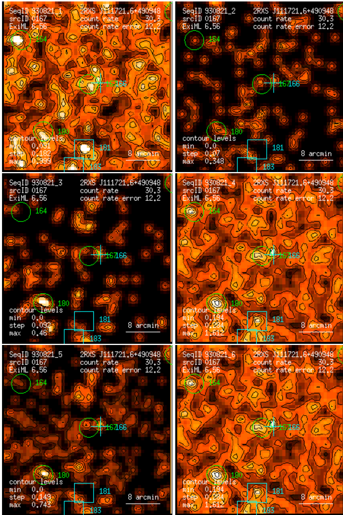
Figure 167: RASS 930821: detection 0167: band rate images, Gaussian filter: (1) PSPC channels 11 – 41, (2) 52 – 90, (3) 91 – 201, (4) 11 – 235, (5) 52 – 201, (6) 11 – 201. Broad band rates in counts/ks. Band rate contour levels in counts/ks/arcmin 2 .
