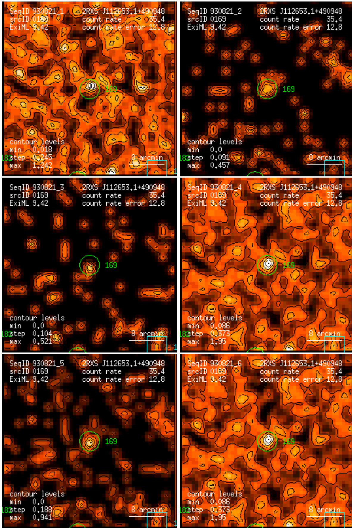
Figure 169: RASS 930821: detection 0169: band rate images, Gaussian filter: (1) PSPC channels 11 – 41, (2) 52 – 90, (3) 91 – 201, (4) 11 – 235, (5) 52 – 201, (6) 11 – 201. Broad band rates in counts/ks. Band rate contour levels in counts/ks/arcmin 2 .
