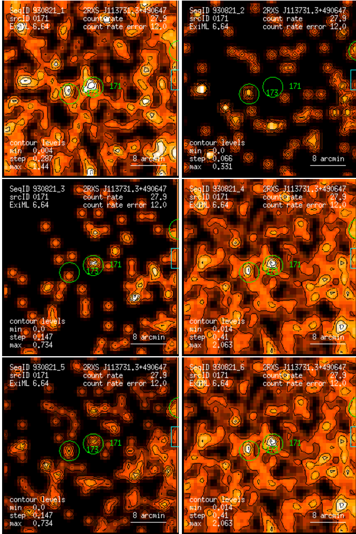
Figure 171: RASS 930821: detection 0171: band rate images, Gaussian filter: (1) PSPC channels 11 – 41, (2) 52 – 90, (3) 91 – 201, (4) 11 – 235, (5) 52 – 201, (6) 11 – 201. Broad band rates in counts/ks. Band rate contour levels in counts/ks/arcmin 2 .
