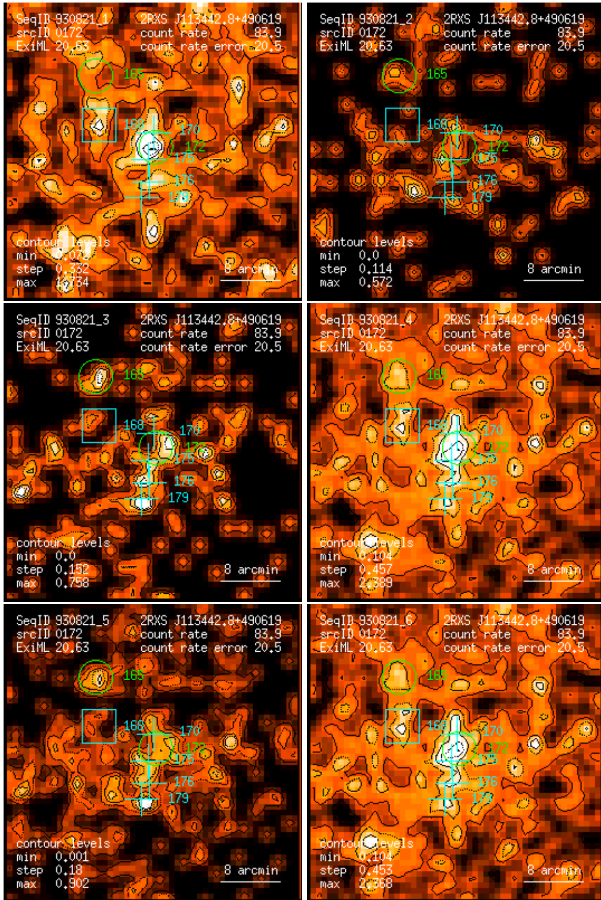
Figure 172: RASS 930821: detection 0172: band rate images, Gaussian filter: (1) PSPC channels 11 – 41, (2) 52 – 90, (3) 91 – 201, (4) 11 – 235, (5) 52 – 201, (6) 11 – 201. Broad band rates in counts/ks. Band rate contour levels in counts/ks/arcmin 2 .
