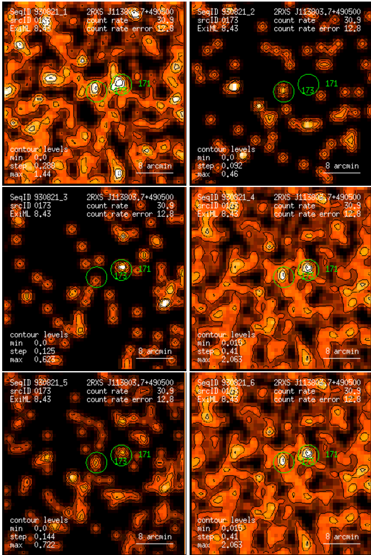
Figure 173: RASS 930821: detection 0173: band rate images, Gaussian filter: (1) PSPC channels 11 – 41, (2) 52 – 90, (3) 91 – 201, (4) 11 – 235, (5) 52 – 201, (6) 11 – 201. Broad band rates in counts/ks. Band rate contour levels in counts/ks/arcmin 2 .
