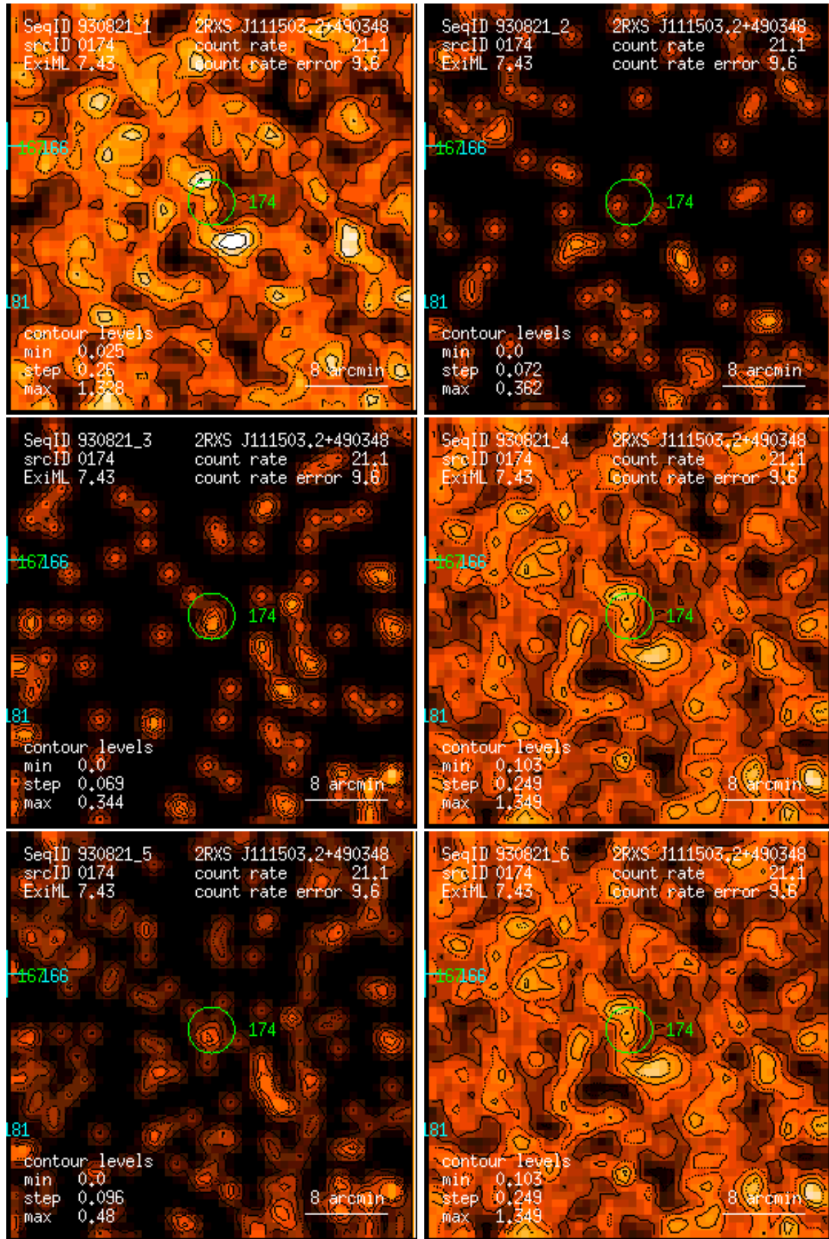
Figure 174: RASS 930821: detection 0174: band rate images, Gaussian filter: (1) PSPC channels 11 – 41, (2) 52 – 90, (3) 91 – 201, (4) 11 – 235, (5) 52 – 201, (6) 11 – 201. Broad band rates in counts/ks. Band rate contour levels in counts/ks/arcmin 2 .
