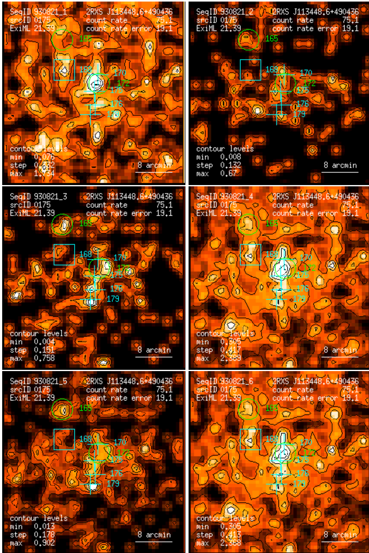
Figure 175: RASS 930821: detection 0175: band rate images, Gaussian filter: (1) PSPC channels 11 – 41, (2) 52 – 90, (3) 91 – 201, (4) 11 – 235, (5) 52 – 201, (6) 11 – 201. Broad band rates in counts/ks. Band rate contour levels in counts/ks/arcmin 2 .
