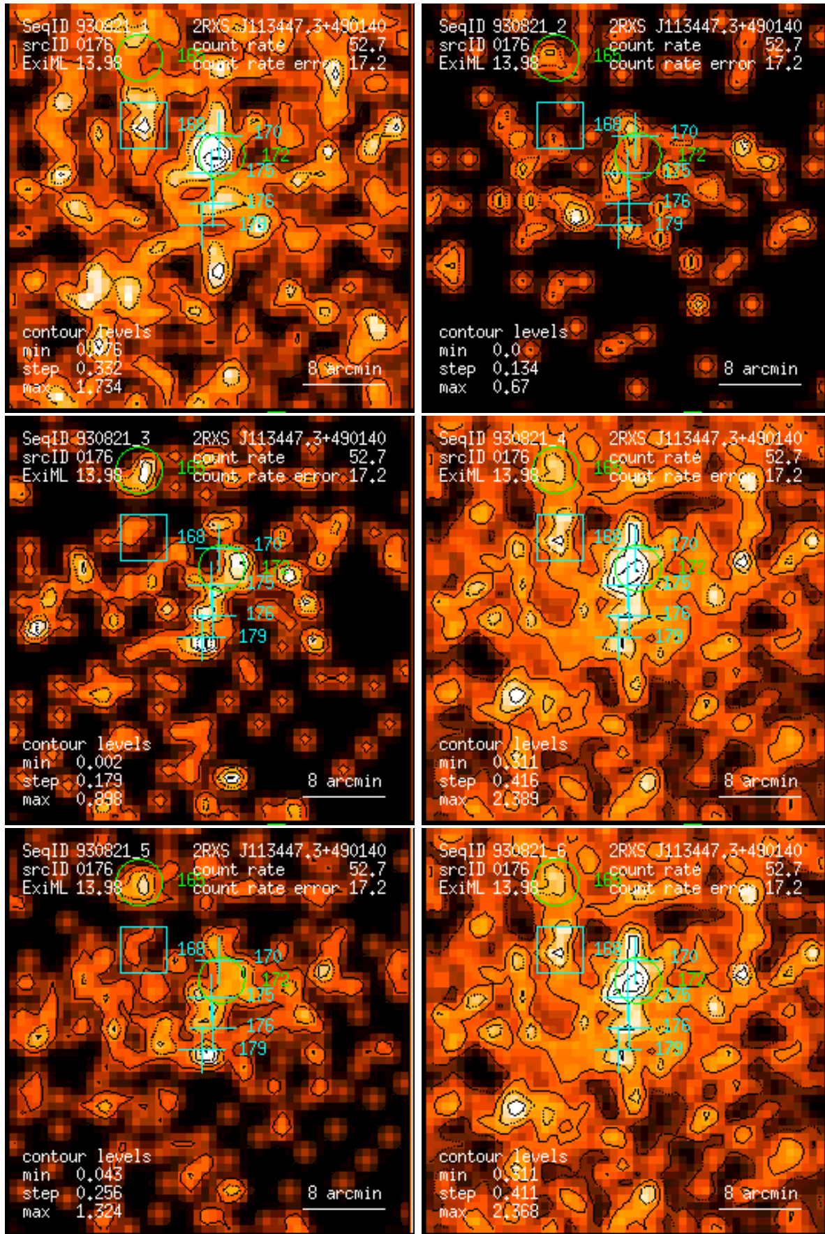
Figure 176: RASS 930821: detection 0176: band rate images, Gaussian filter: (1) PSPC channels 11 – 41, (2) 52 – 90, (3) 91 – 201, (4) 11 – 235, (5) 52 – 201, (6) 11 – 201. Broad band rates in counts/ks. Band rate contour levels in counts/ks/arcmin 2 .
