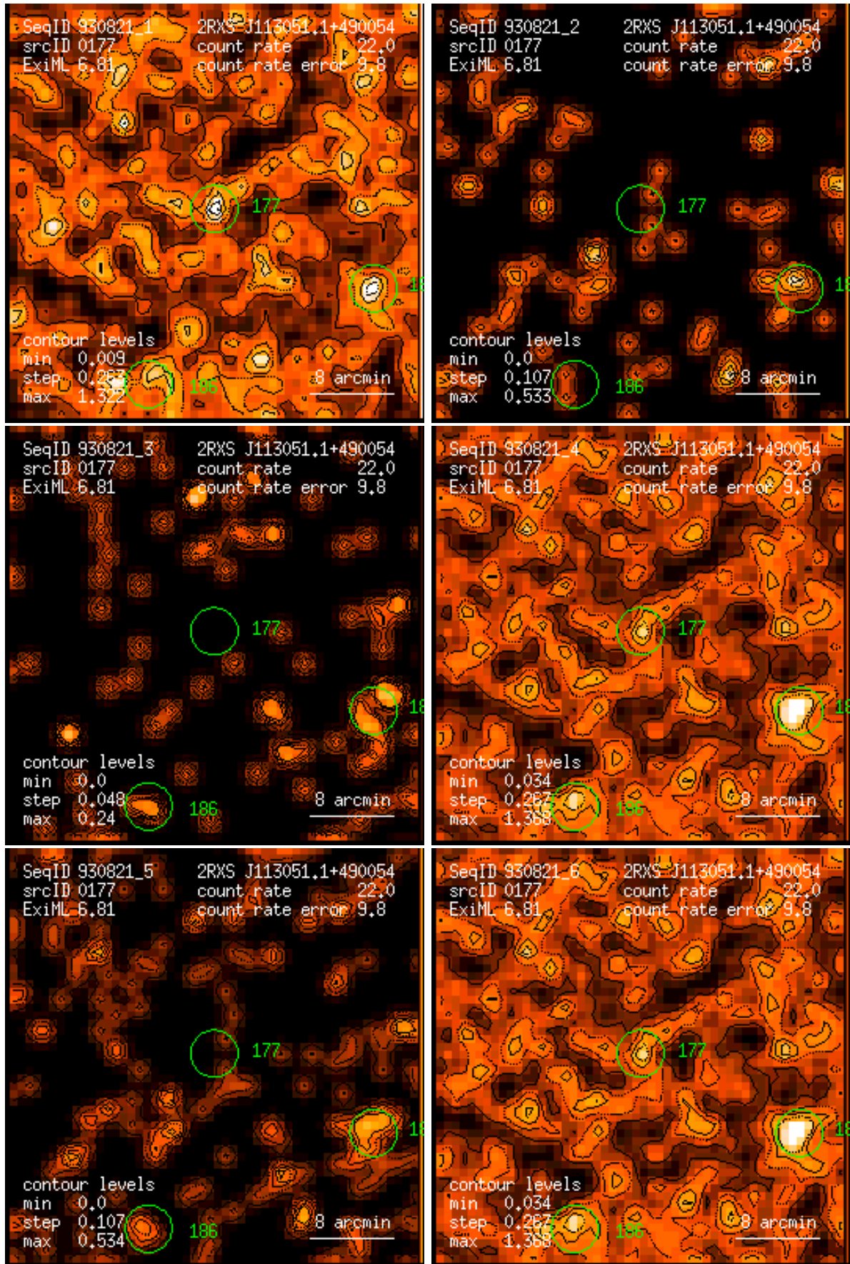
Figure 177: RASS 930821: detection 0177: band rate images, Gaussian filter: (1) PSPC channels 11 – 41, (2) 52 – 90, (3) 91 – 201, (4) 11 – 235, (5) 52 – 201, (6) 11 – 201. Broad band rates in counts/ks. Band rate contour levels in counts/ks/arcmin 2 .
