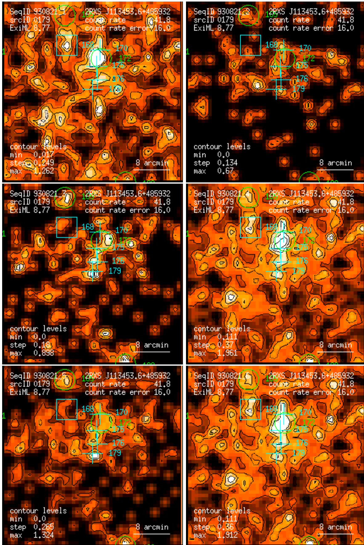
Figure 179: RASS 930821: detection 0179: band rate images, Gaussian filter: (1) PSPC channels 11 – 41, (2) 52 – 90, (3) 91 – 201, (4) 11 – 235, (5) 52 – 201, (6) 11 – 201. Broad band rates in counts/ks. Band rate contour levels in counts/ks/arcmin 2 .
