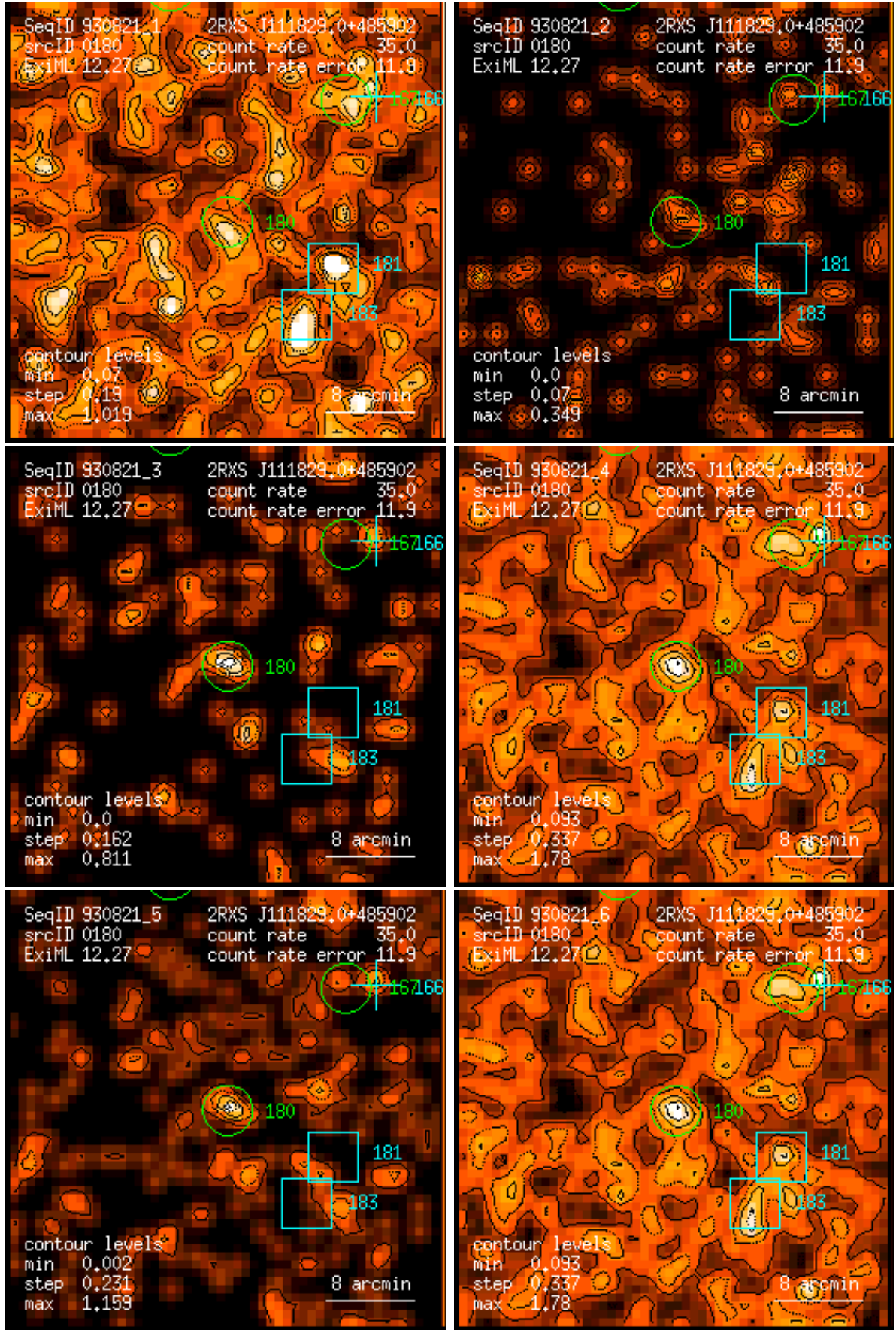
Figure 180: RASS 930821: detection 0180: band rate images, Gaussian filter: (1) PSPC channels 11 – 41, (2) 52 – 90, (3) 91 – 201, (4) 11 – 235, (5) 52 – 201, (6) 11 – 201. Broad band rates in counts/ks. Band rate contour levels in counts/ks/arcmin 2 .
