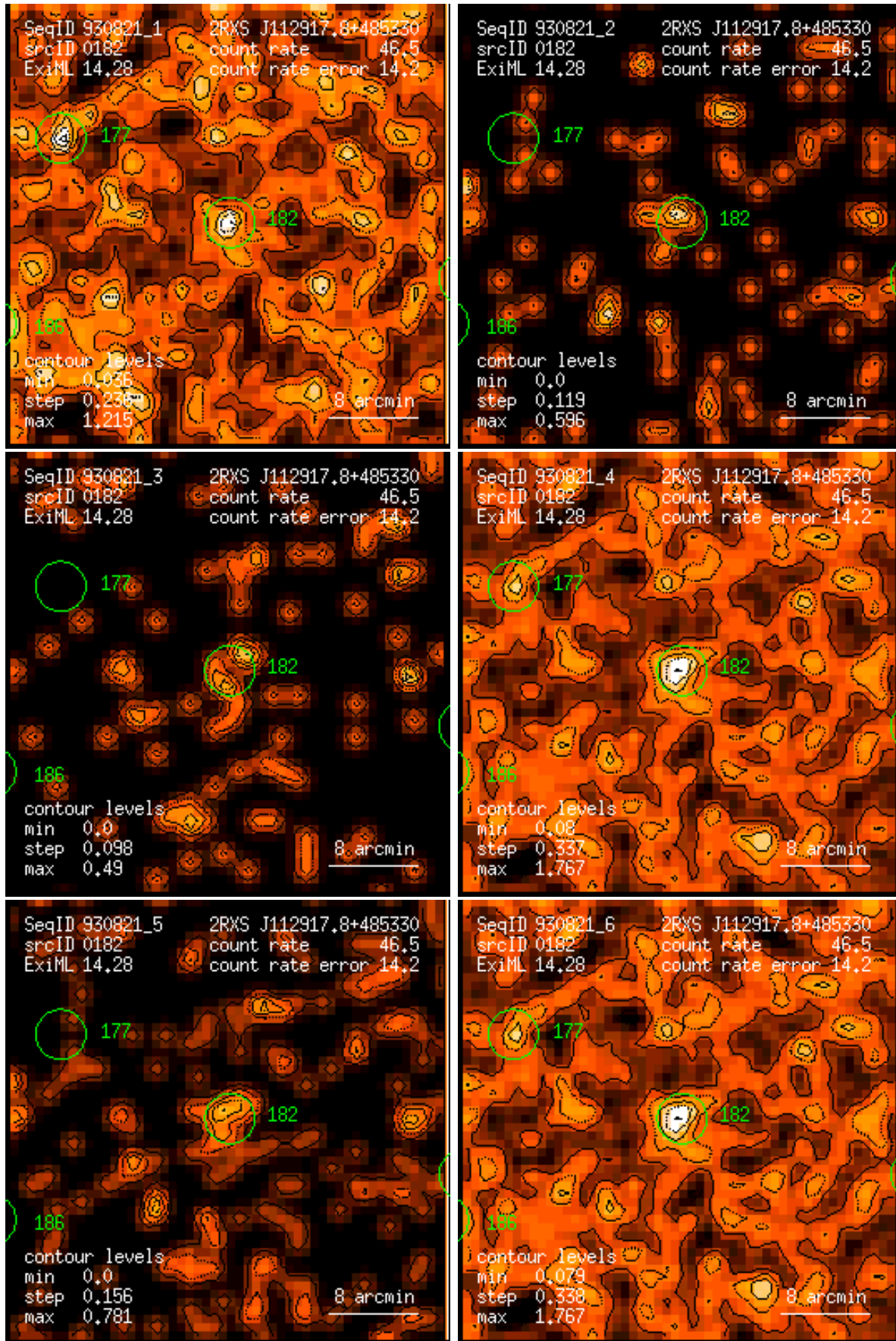
Figure 182: RASS 930821: detection 0182: band rate images, Gaussian filter: (1) PSPC channels 11 – 41, (2) 52 – 90, (3) 91 – 201, (4) 11 – 235, (5) 52 – 201, (6) 11 – 201. Broad band rates in counts/ks. Band rate contour levels in counts/ks/arcmin 2 .
