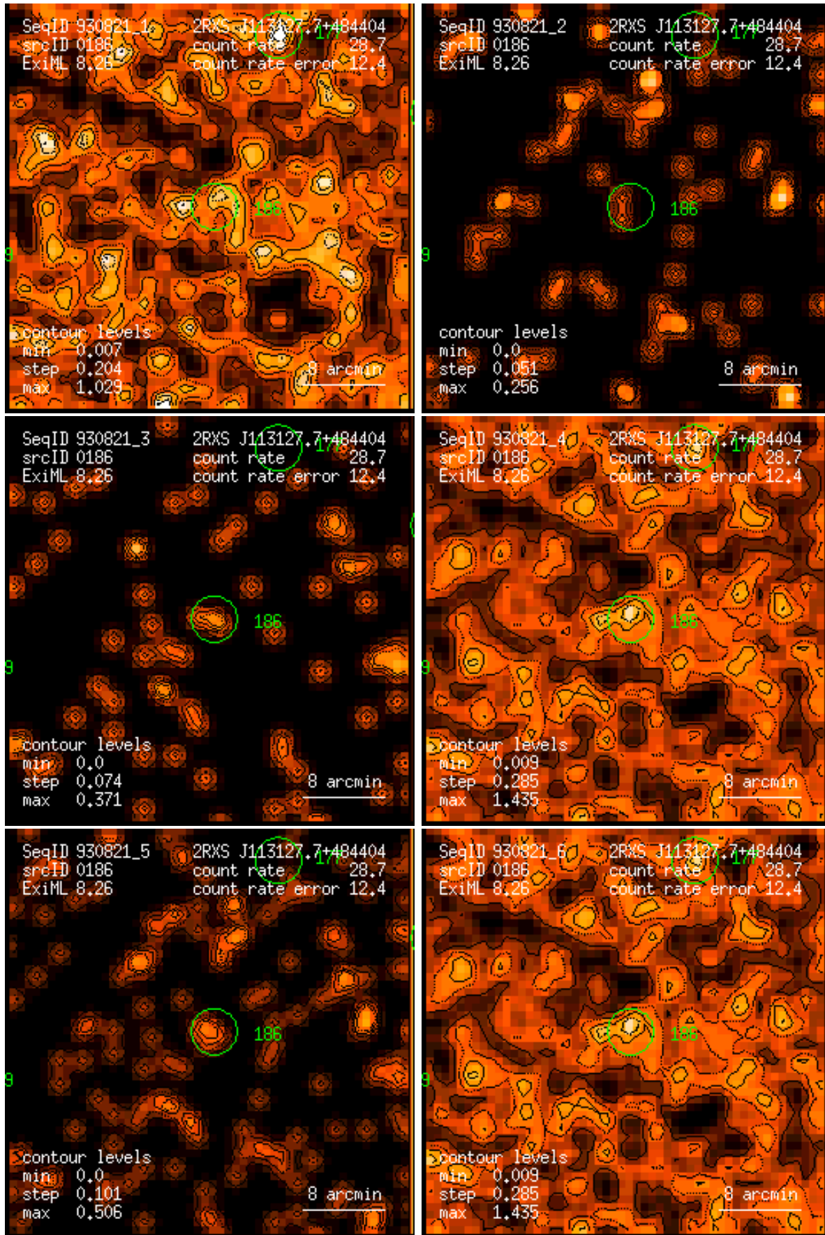
Figure 186: RASS 930821: detection 0186: band rate images, Gaussian filter: (1) PSPC channels 11 – 41, (2) 52 – 90, (3) 91 – 201, (4) 11 – 235, (5) 52 – 201, (6) 11 – 201. Broad band rates in counts/ks. Band rate contour levels in counts/ks/arcmin 2 .
