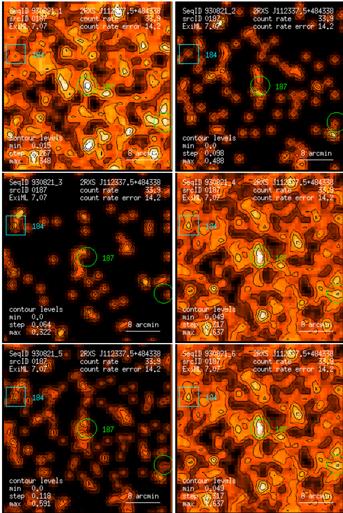
Figure 187: RASS 930821: detection 0187: band rate images, Gaussian filter: (1) PSPC channels 11 – 41, (2) 52 – 90, (3) 91 – 201, (4) 11 – 235, (5) 52 – 201, (6) 11 – 201. Broad band rates in counts/ks. Band rate contour levels in counts/ks/arcmin 2 .
