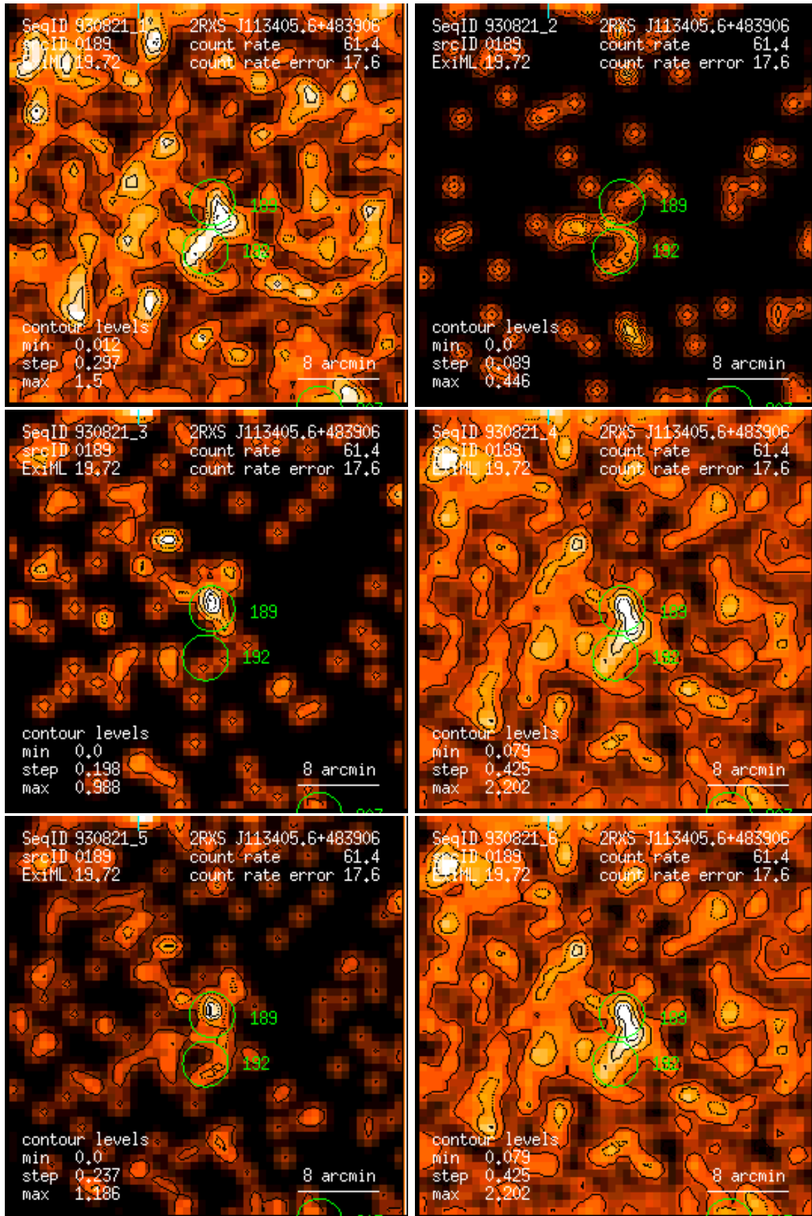
Figure 189: RASS 930821: detection 0189: band rate images, Gaussian filter: (1) PSPC channels 11 – 41, (2) 52 – 90, (3) 91 – 201, (4) 11 – 235, (5) 52 – 201, (6) 11 – 201. Broad band rates in counts/ks. Band rate contour levels in counts/ks/arcmin 2 .
